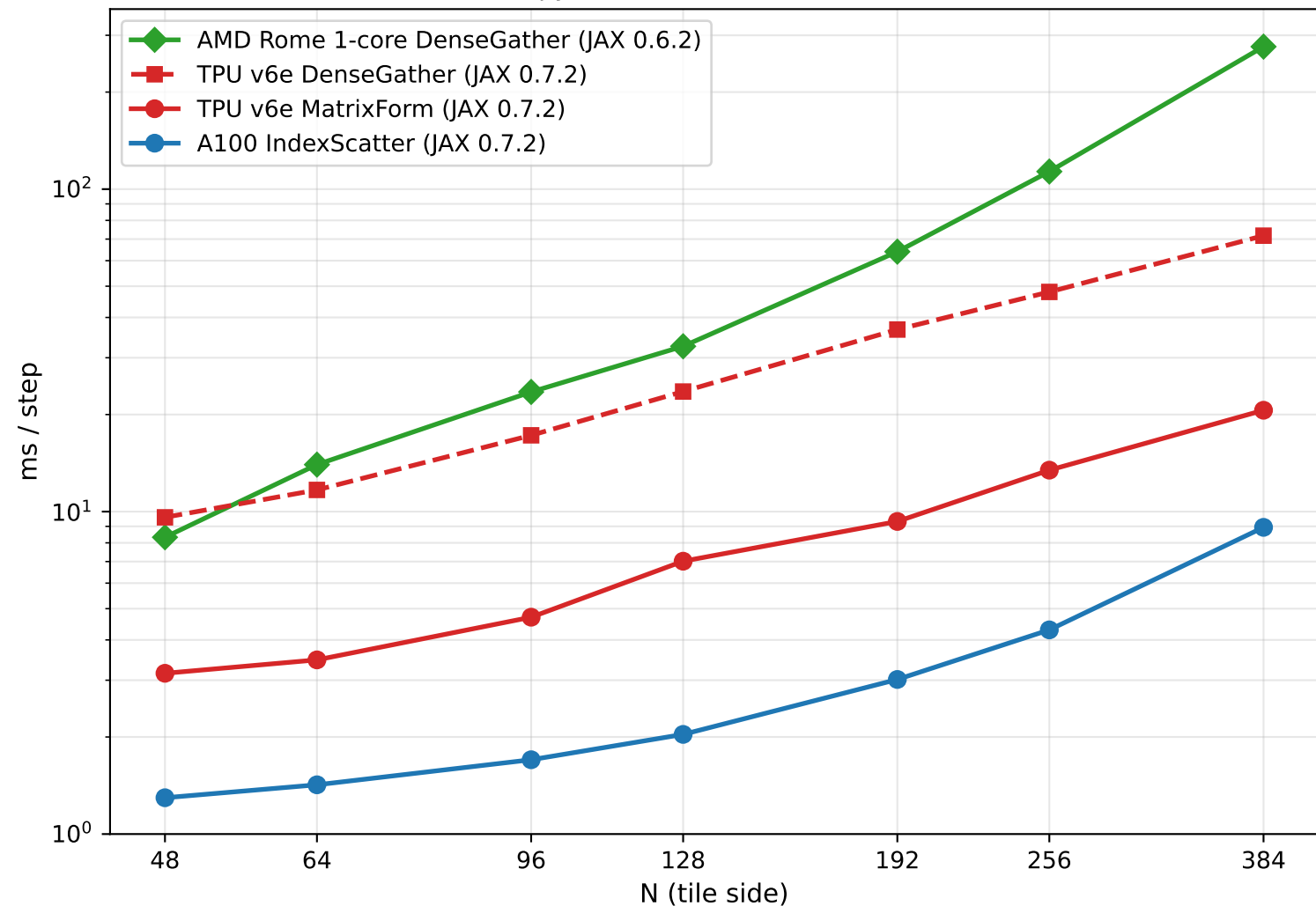
JAX FP32 (ms/RK4 step) Performance on Galewsky Barotropic Instability Test for AMD Epyc (Rome) CPU, A100 GPU, V6e TPU
