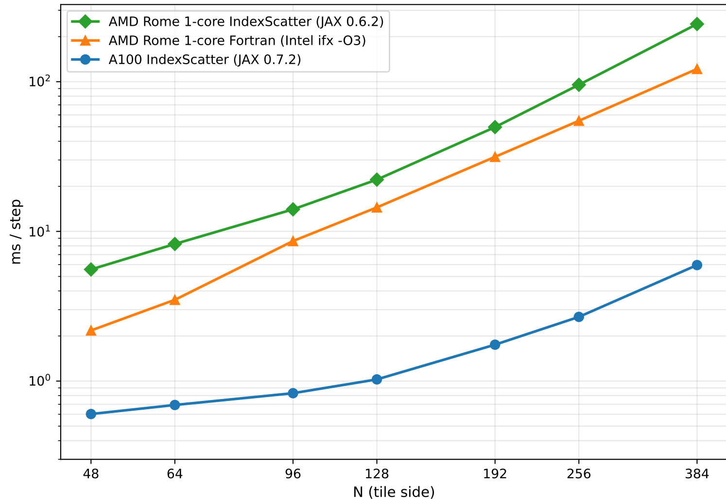
FP64 (ms/RK4 step) Performance on gauss3 (Rotating Gaussian Hill, Linear SWE) for AMD Epyc (Rome) CPU [Fortran + JAX] and A100 GPU [JAX]
