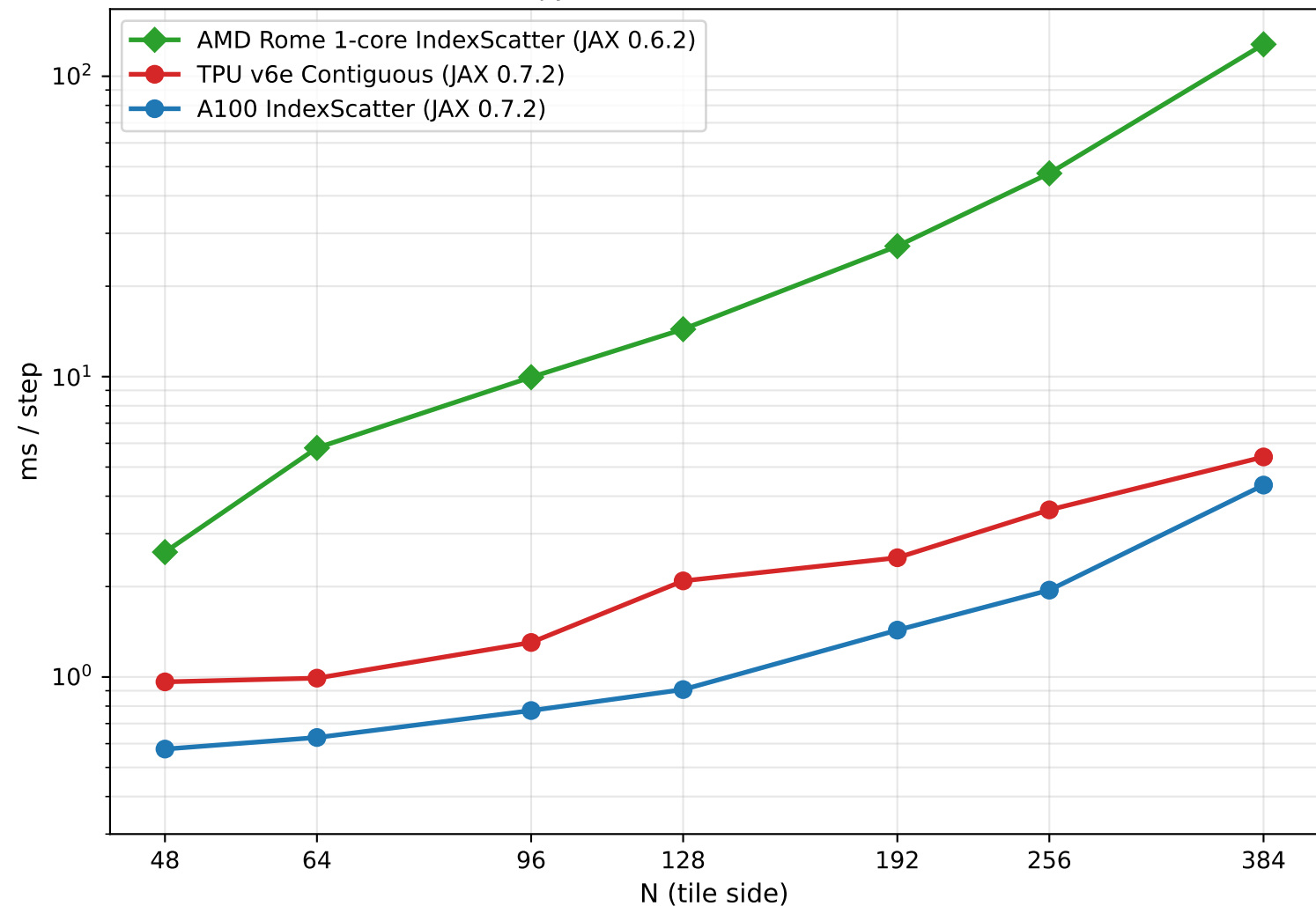
JAX FP32 (ms/RK4 step) Performance on gauss3 (Rotating Gaussian Hill, Linear SWE) for AMD Epyc (Rome) CPU, A100 GPU, V6e TPU
