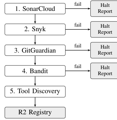
Fig. 1. Security pipeline publish workflow. Each of the four scanning stages halts immediately on a critical finding and returns a consolidated report to the developer; repositories clearing all five stages proceed to tool discovery and R2 registration.
