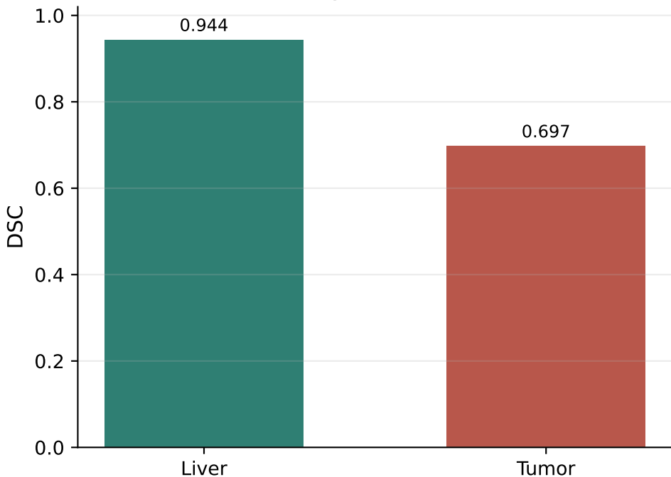
Held-Out Test Segmentation Performance
