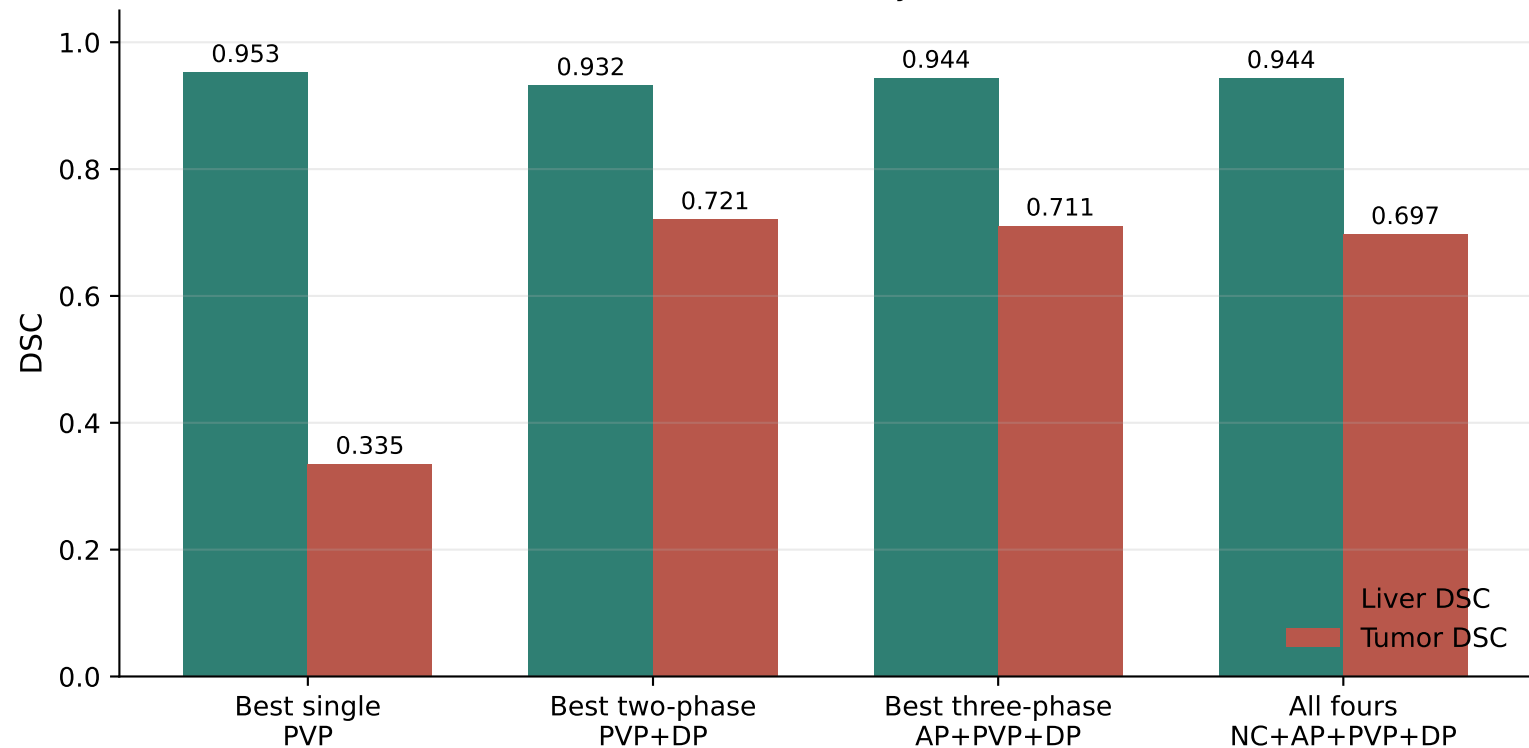
Best Phase Subsets by Tumor DSC
