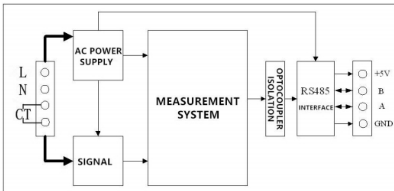
Picture 3.2 PZEM-016 Functional block diagram
