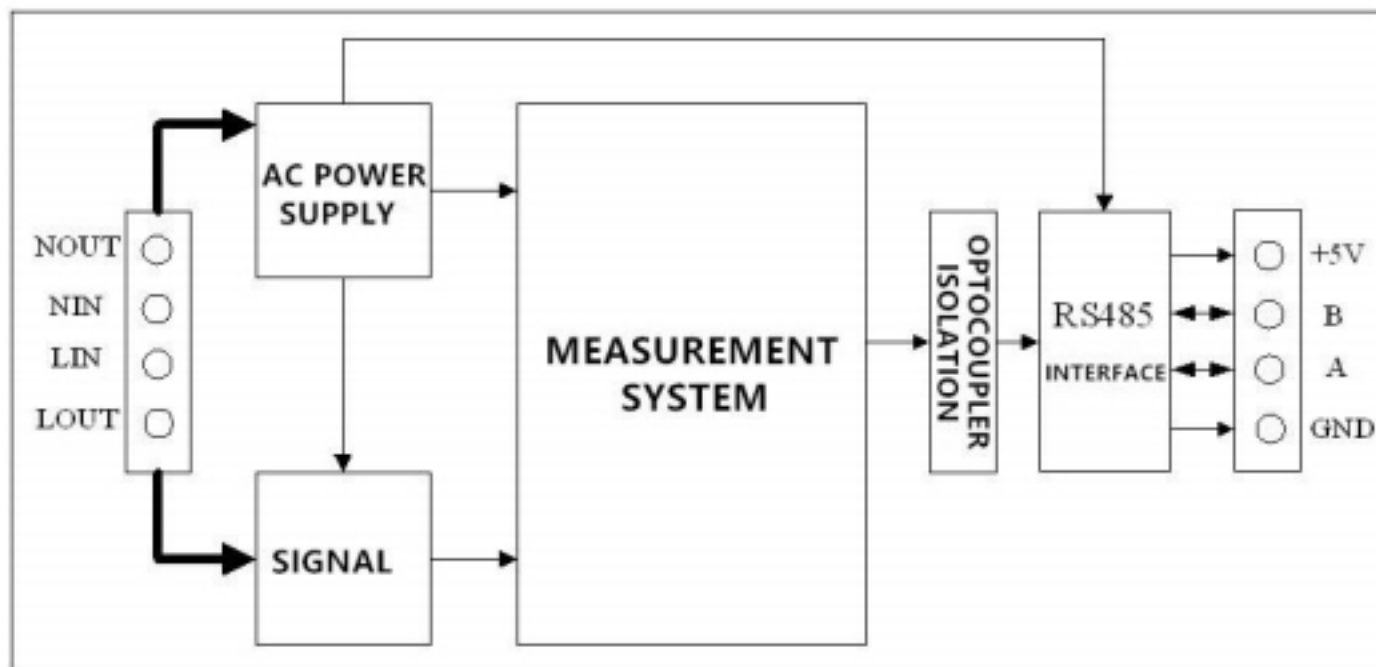
Picture 3.1 PZEM-014 Functional block diagram
