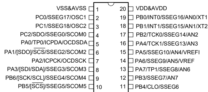
HT66F0175/HT66V0175 20 SOP-A/SSOP-A
