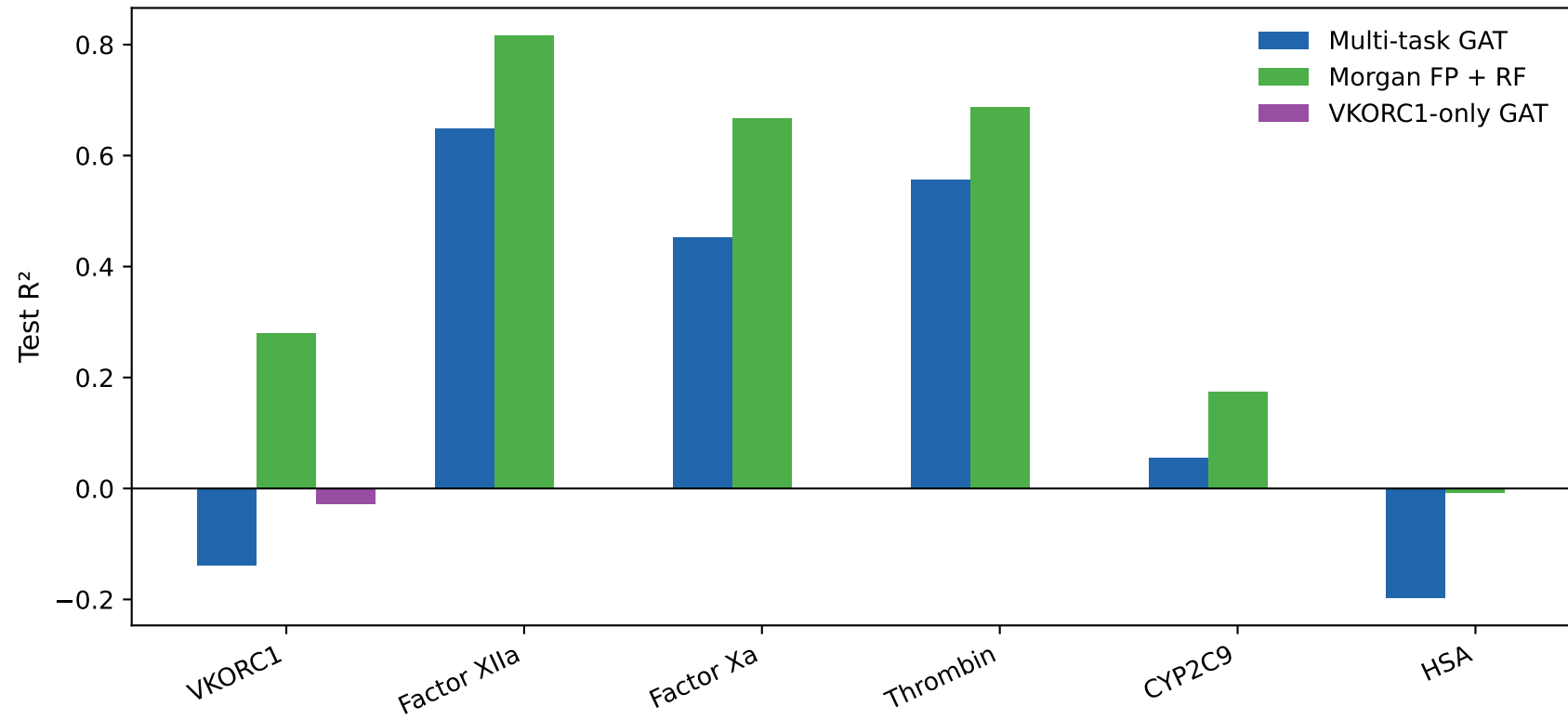
Figure S2. Model comparison (Murcko scaffold hold-out)
