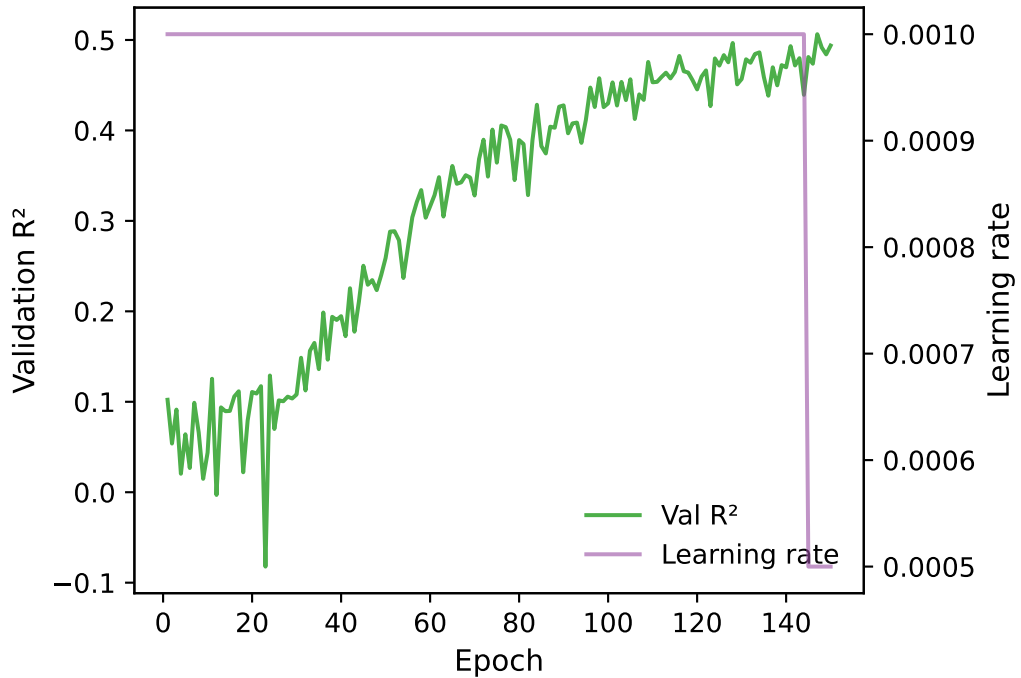
Validation R 2 and LR schedule
