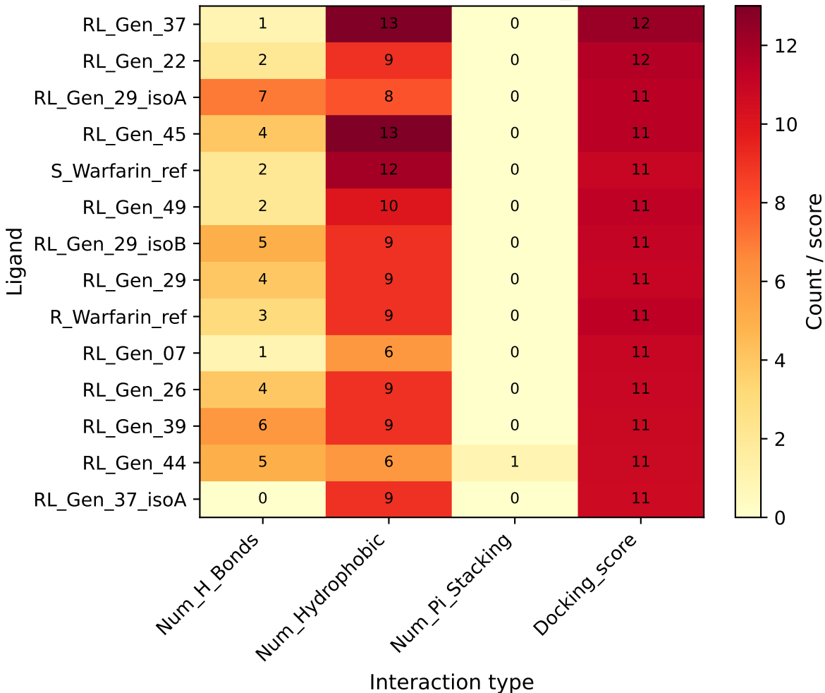
VKORC1 interaction fingerprint (top RL_Gen + references)
