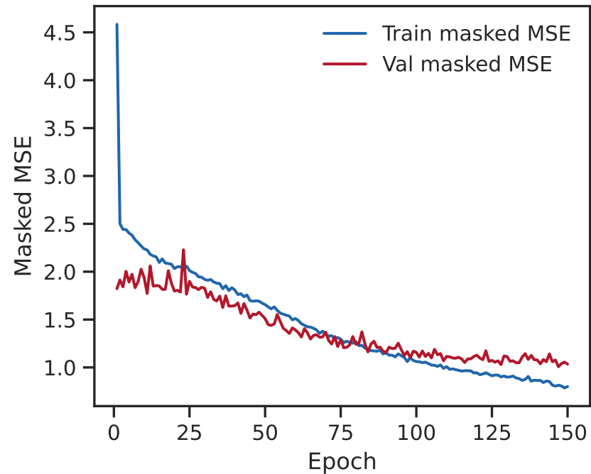
Multi-task GAT training
