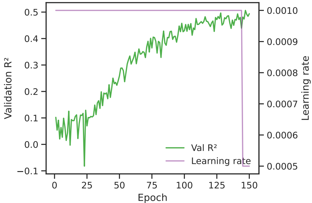
Validation R 2 and LR schedule
