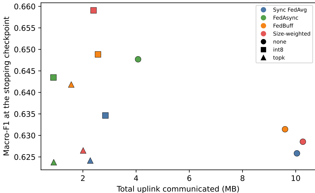
Bot-IoT: communication versus accuracy
