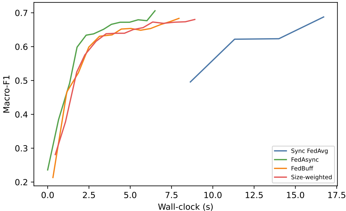
N-BaloT: convergence (mixed network, \alpha=0.5 )
