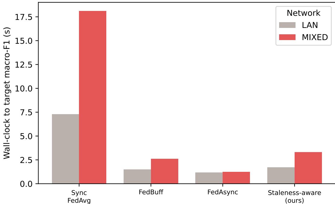
botiot: wall-clock to target, LAN vs mixed network
