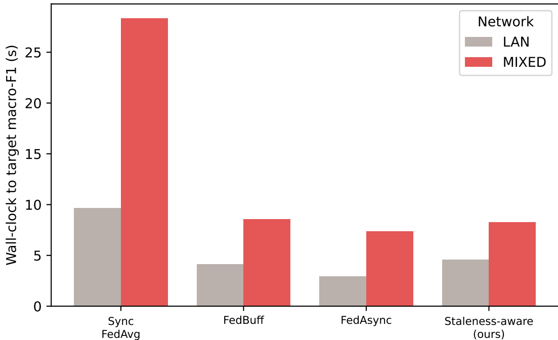
nbaiot: wall-clock to target, LAN vs mixed network
