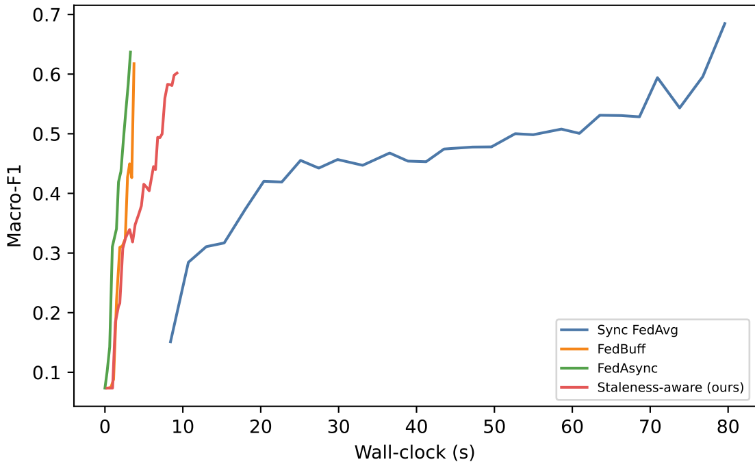
cicids2017: convergence (mixed network, \alpha=0.5 )
