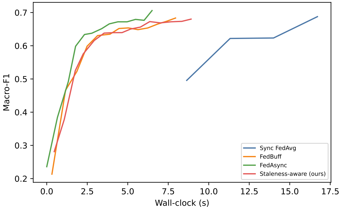
nbaiot: convergence (mixed network, \alpha=0.5 )
