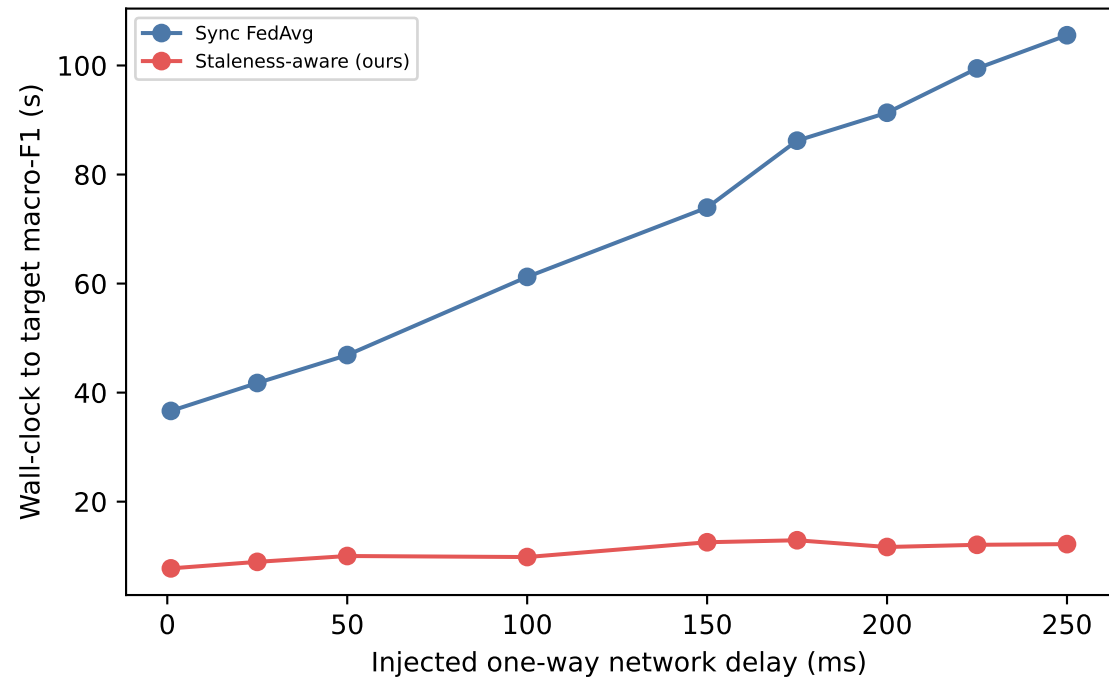
cicids2017: sync vs staleness crossover vs delay
