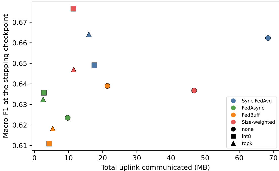
CICIDS2017: communication versus accuracy
