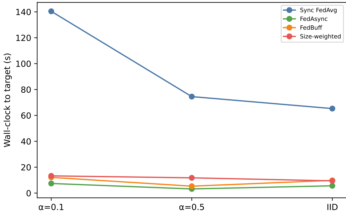
CICIDS2017: wall-clock to target against label skew (mixed network)
