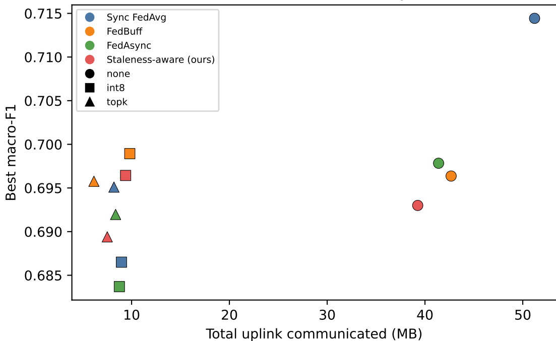
nbaiot: communication-accuracy trade-off
