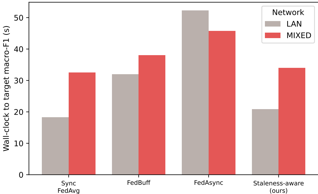
botiot: async pays off under network heterogeneity
