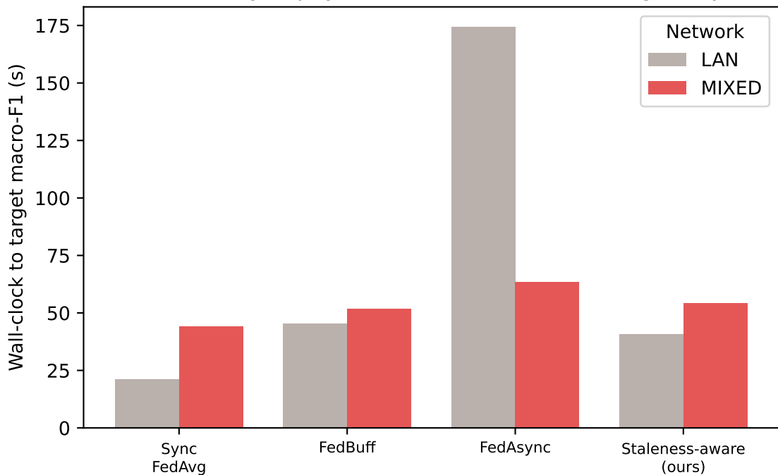
nbaiot: async pays off under network heterogeneity
