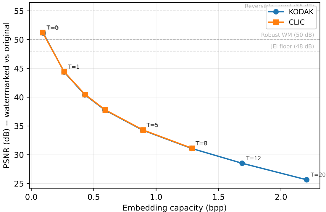
QFormer-RevMark: PSNR-vs-capacity (T sweep)
