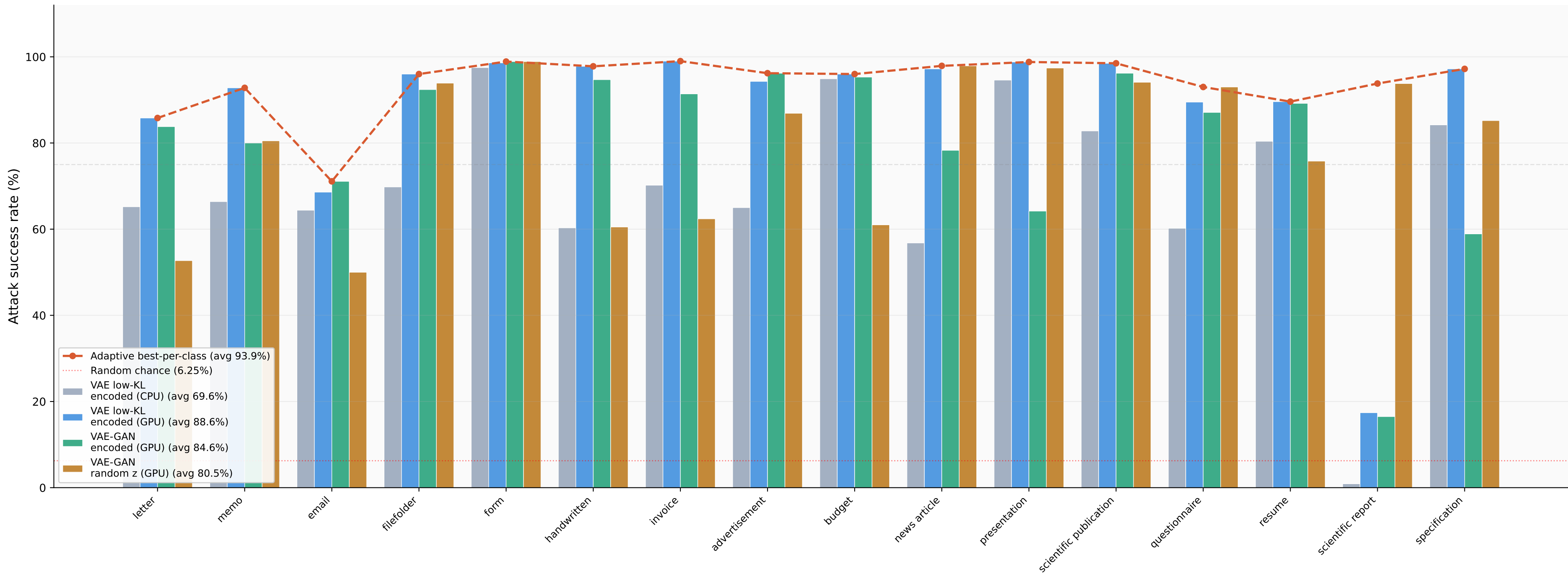
Attack success rate per class — all methods comparison (134 documents per source class, equal evaluation)
