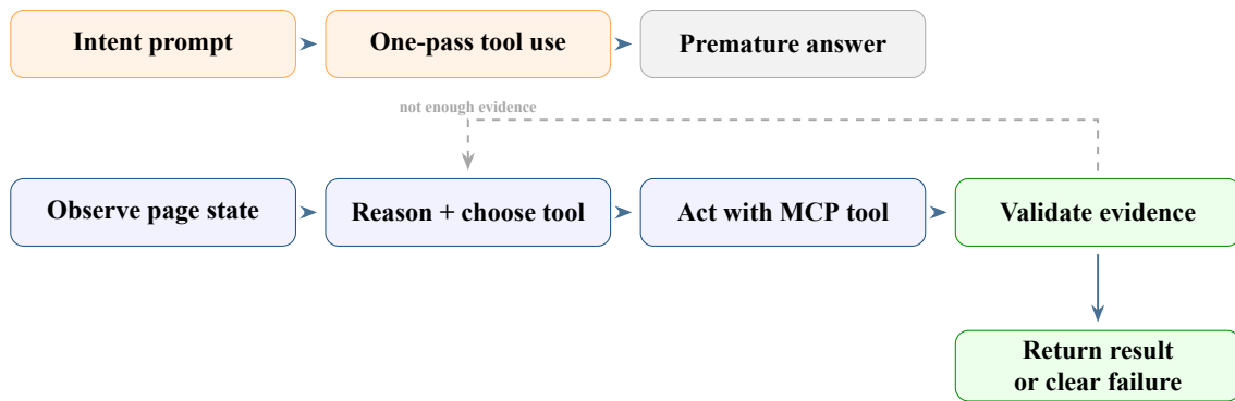
Figure 5.11: Prompt evolution from one-pass intent prompts to evidence-driven agent loops.
