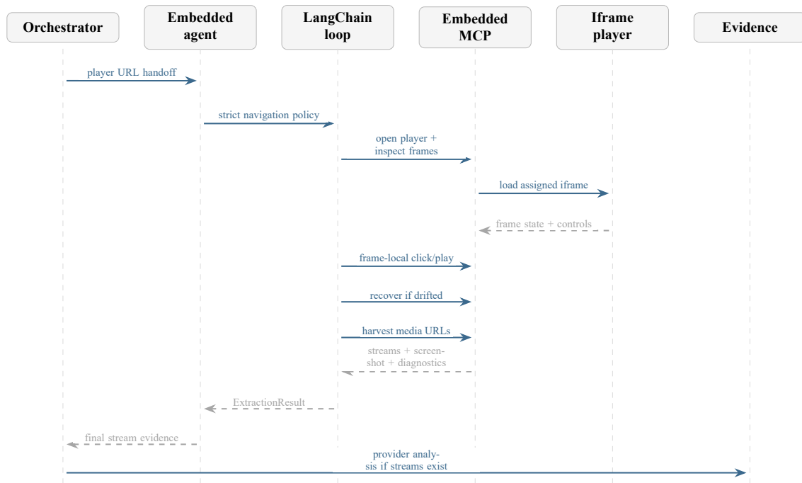
Figure 4.18: Embedded-agent sequence: stay in the player context and harvest final media evidence.
