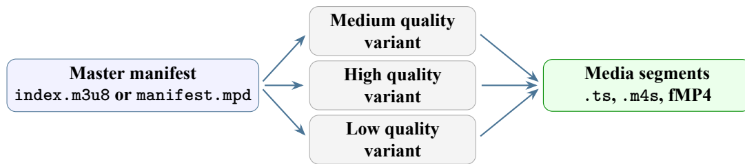
Figure 3.5: Simplified adaptive streaming hierarchy used by HLS and MPEG-DASH.
