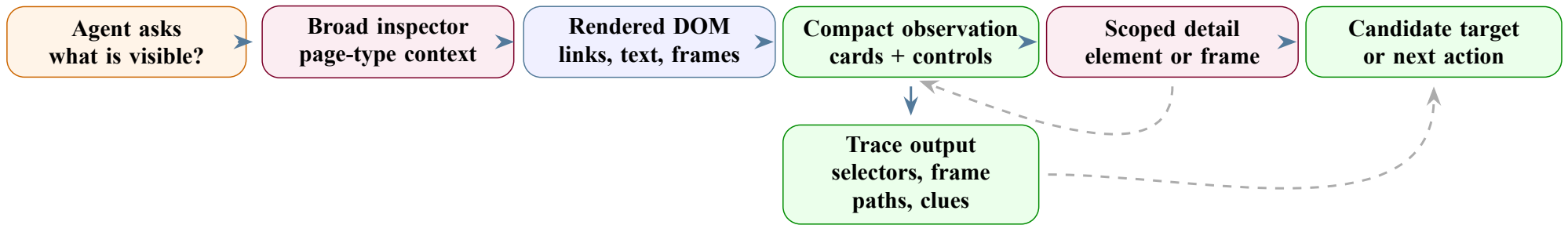
Figure 20: Inspection and context-retrieval flow from rendered DOM observation to scoped targets.
