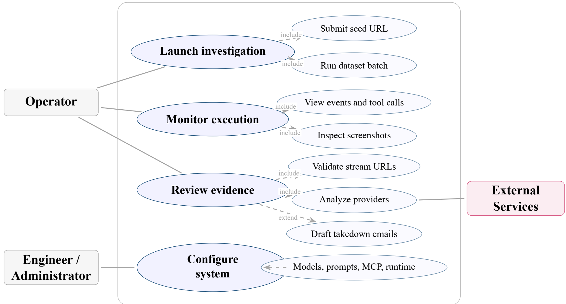
Figure 1: Use-case overview of the evidence-collection platform.
