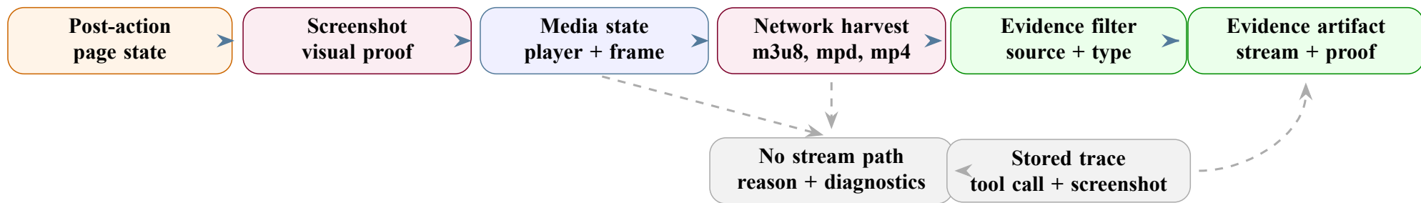
Figure 22: Evidence and media-extraction flow from page state to reviewable artifacts.
