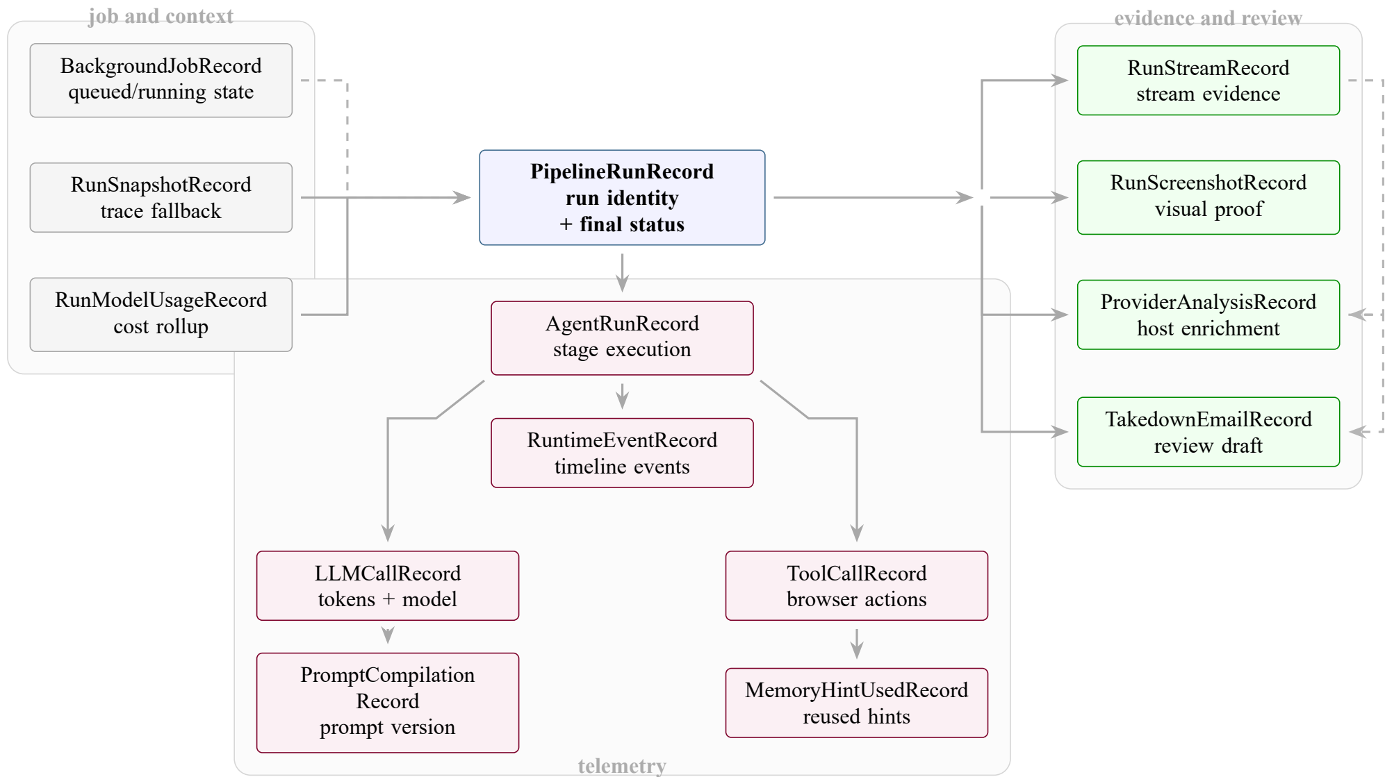
Figure 24: Persistence model for run evidence, telemetry, and review outputs.
