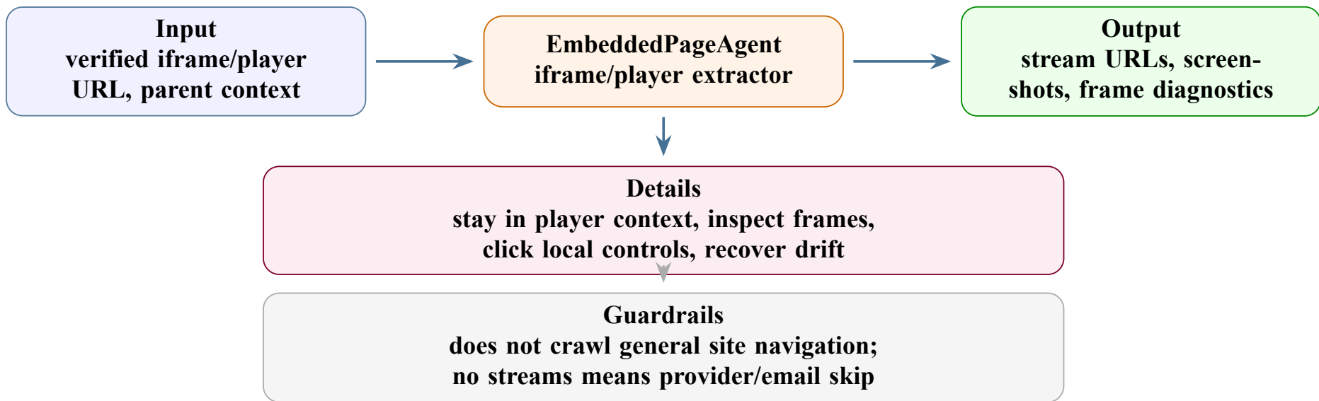
Figure 15: Embedded-page-agent design card.
