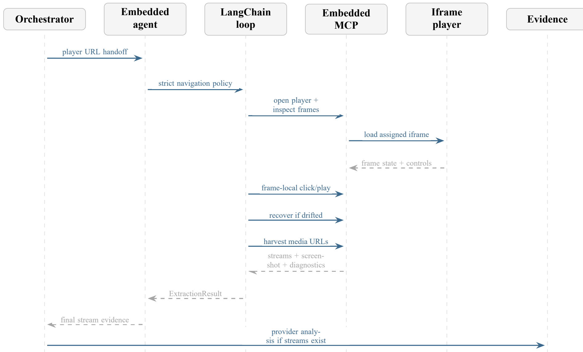
Figure 16: Embedded-agent sequence: stay in the player context and harvest final media evidence.
