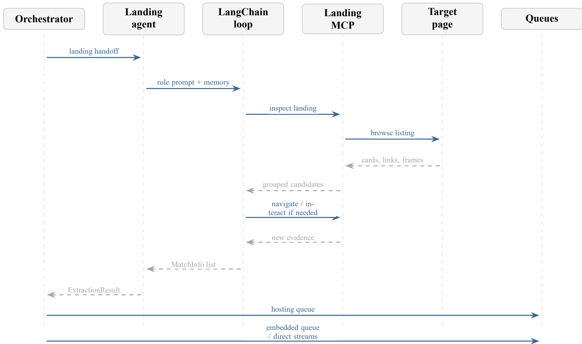
Figure 12: Landing-agent sequence: convert listing-page evidence into downstream queues.
