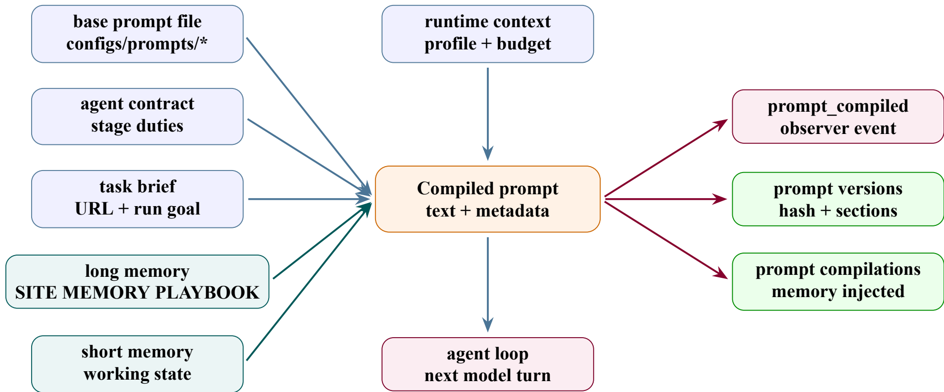
Figure 6: Prompt compilation and memory inputs for each browser-facing specialist.
