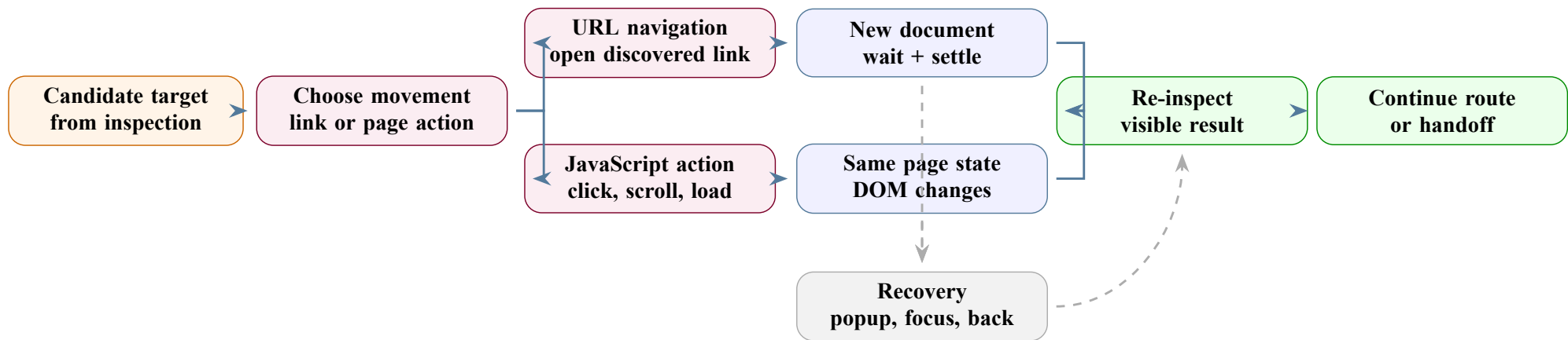
Figure 21: Navigation flow split between direct URL navigation and JavaScript-driven page interaction.
