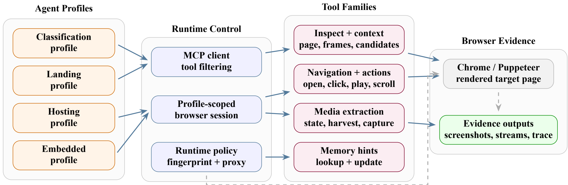
Figure 18: Profile-scoped MCP browser tooling and runtime controls used by OWC agents.
