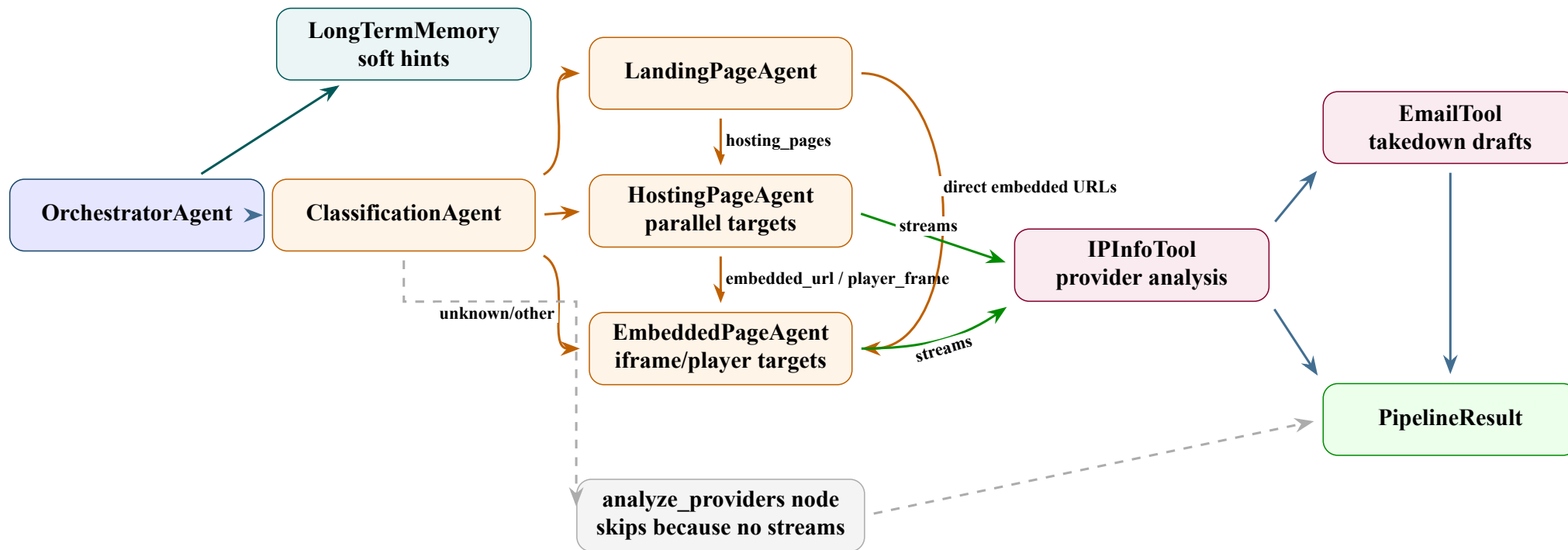
Figure 5: Agent interconnection graph showing orchestrator-owned routing and specialist responsibilities.
