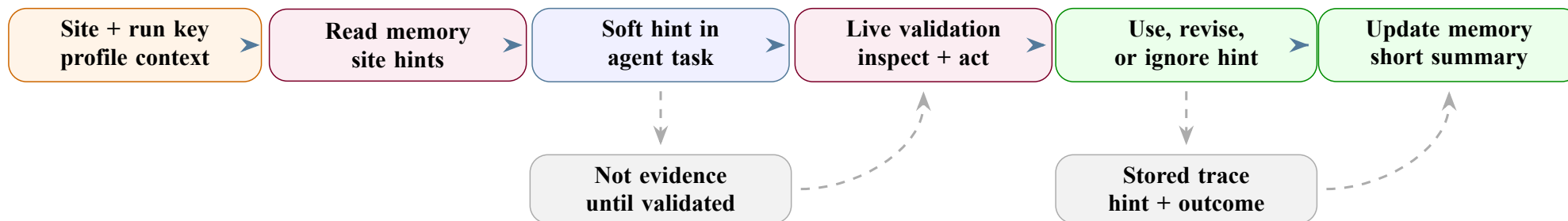
Figure 23: Memory-tool flow showing hints as guidance that must be validated live.
