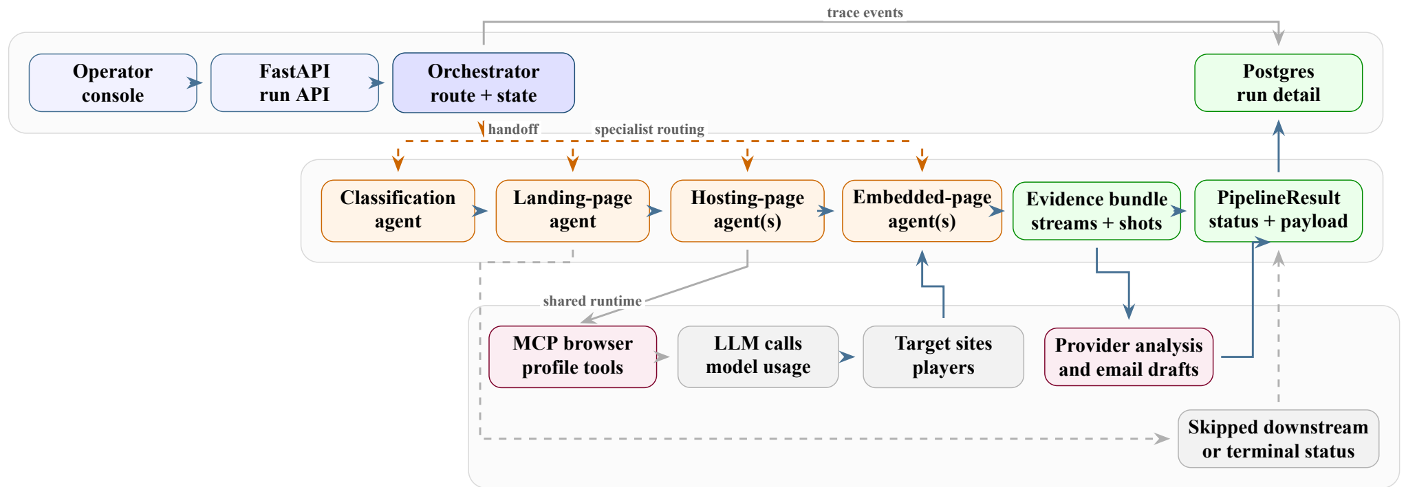
Figure 3: End-to-end agent architecture at workflow scale.
