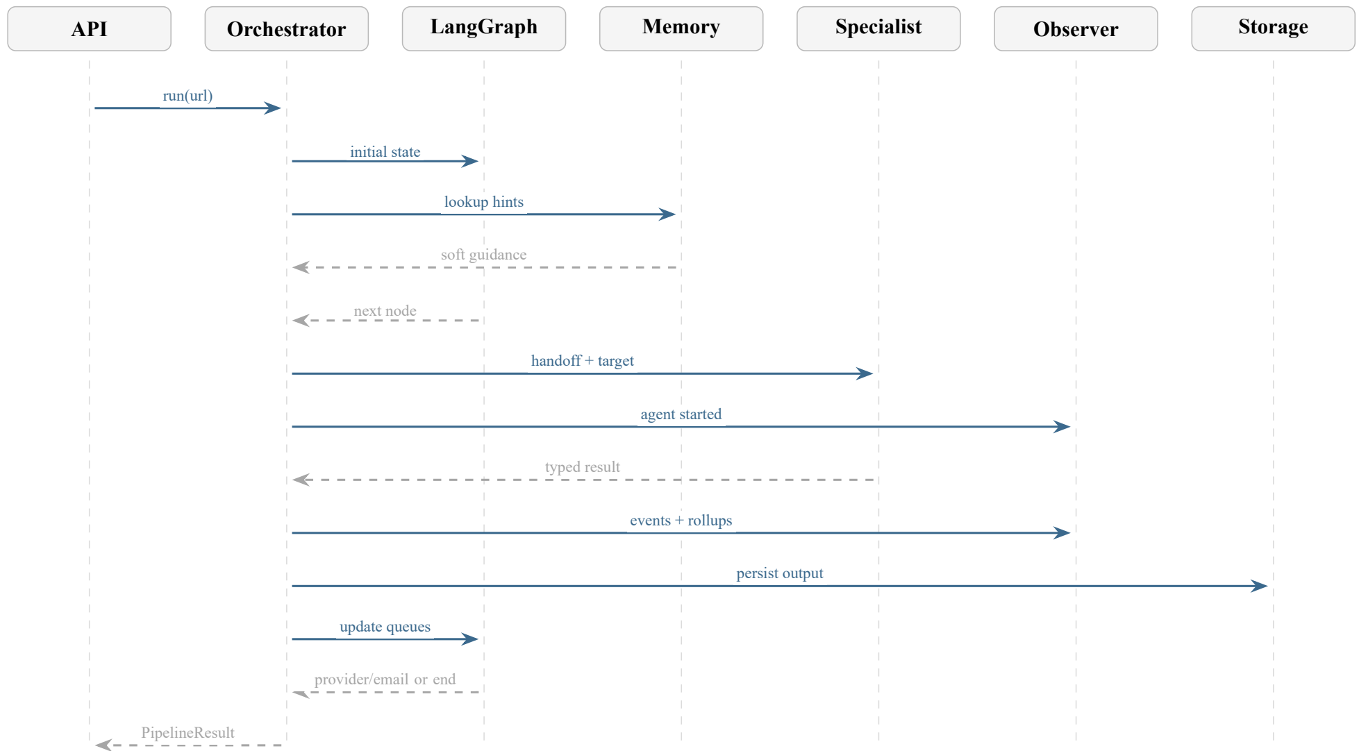
Figure 8: Sequence diagram for orchestrator handoff, trace recording, and route updates.
