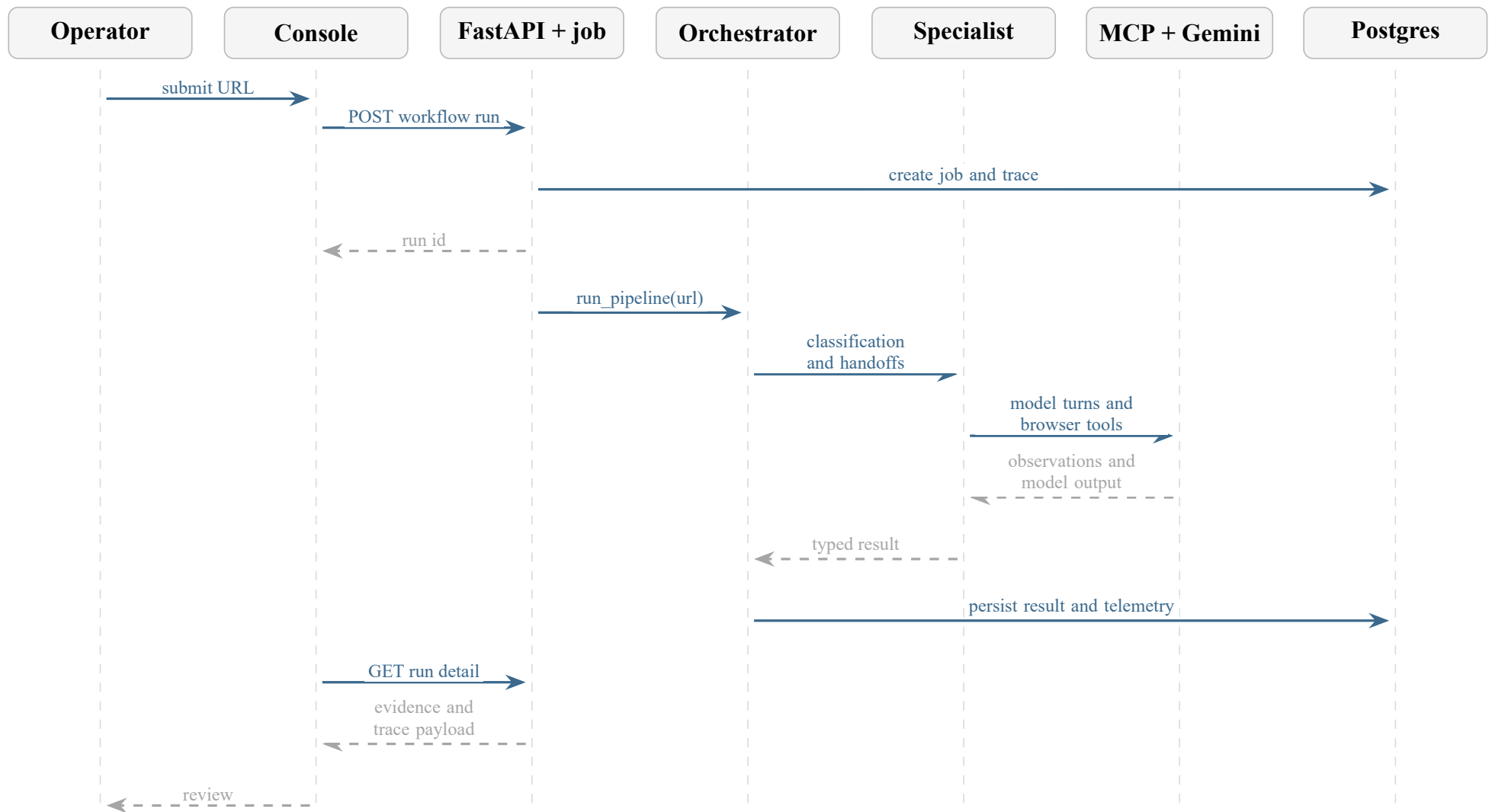
Figure 4: Sequence diagram for launching, executing, persisting, and reviewing a workflow run.
