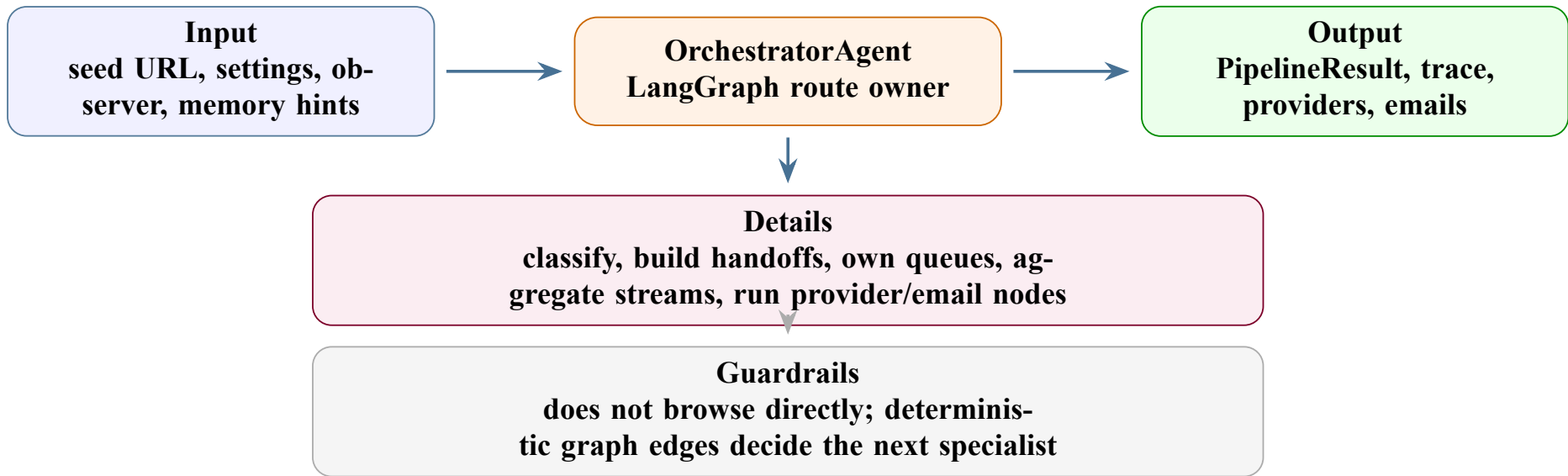
Figure 7: Orchestrator-agent design card.
