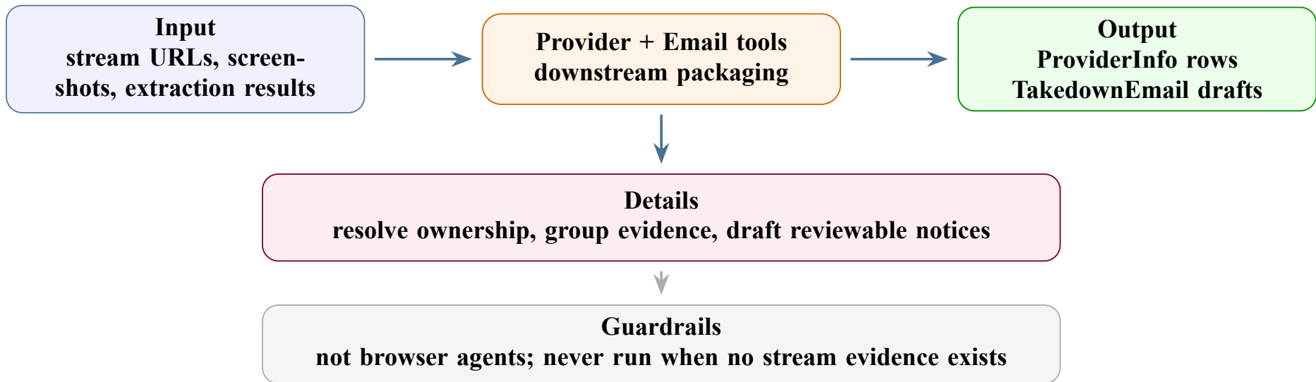
Figure 17: Provider-analysis and email-generation design card.
