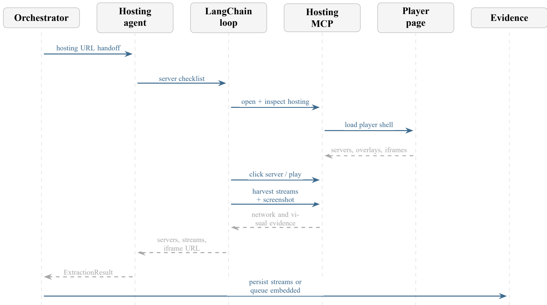
Figure 14: Hosting-agent sequence: activate watch pages and return stream or iframe evidence.
