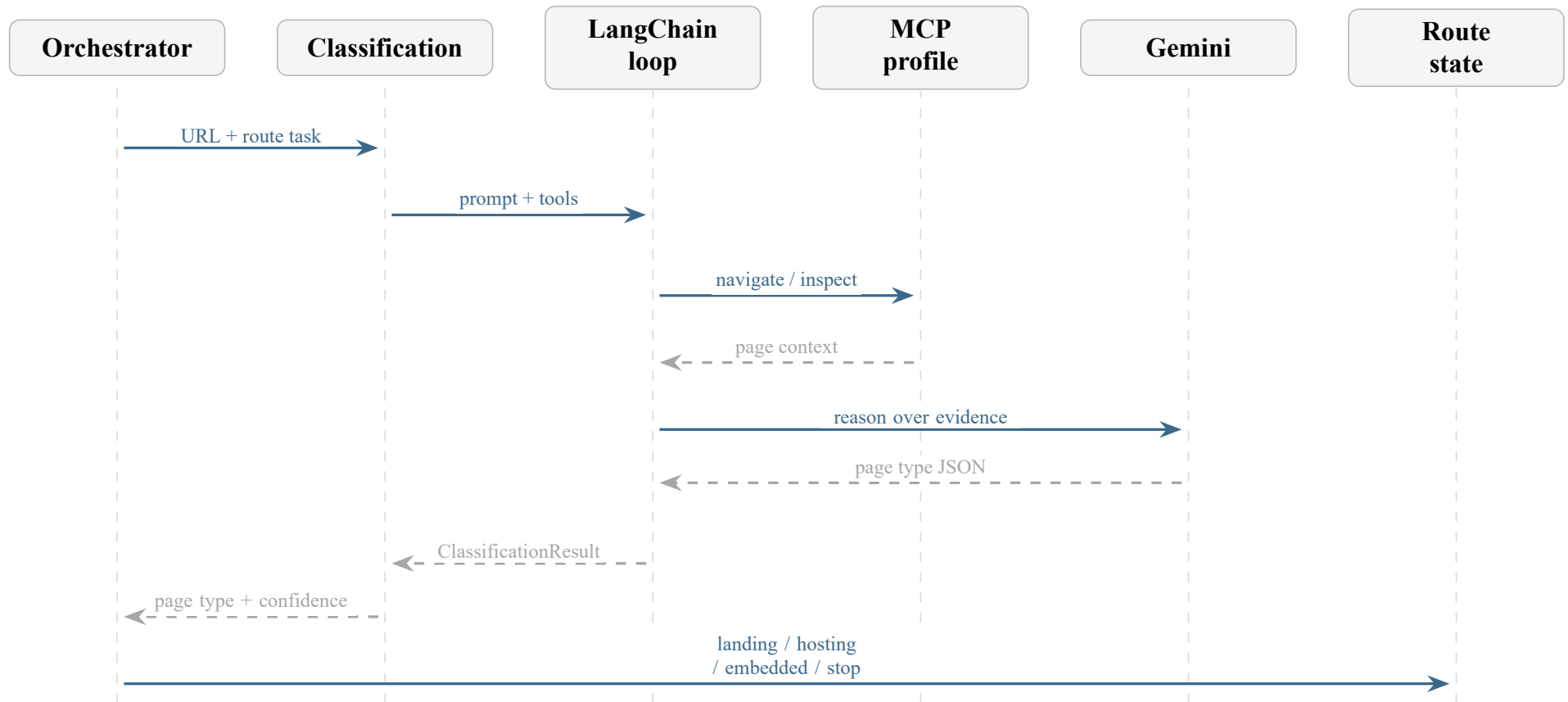
Figure 10: Classification-agent sequence: inspect page state and return a routing decision.
