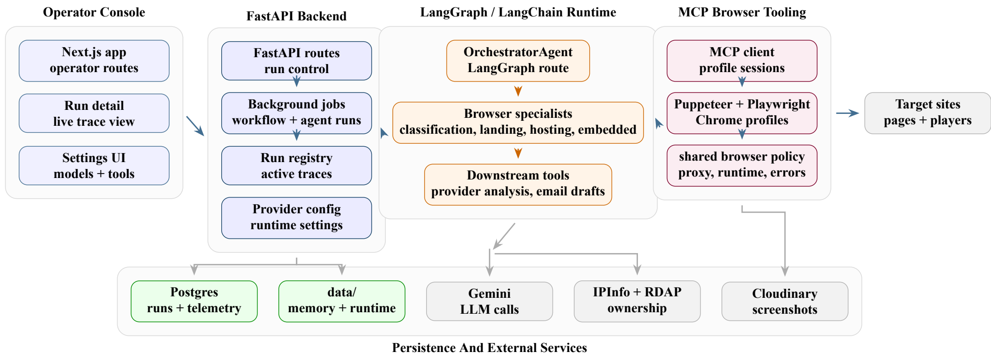
Figure 2: Component architecture linking the operator console, backend, agent runtime, MCP tooling, persistence, and external services.
