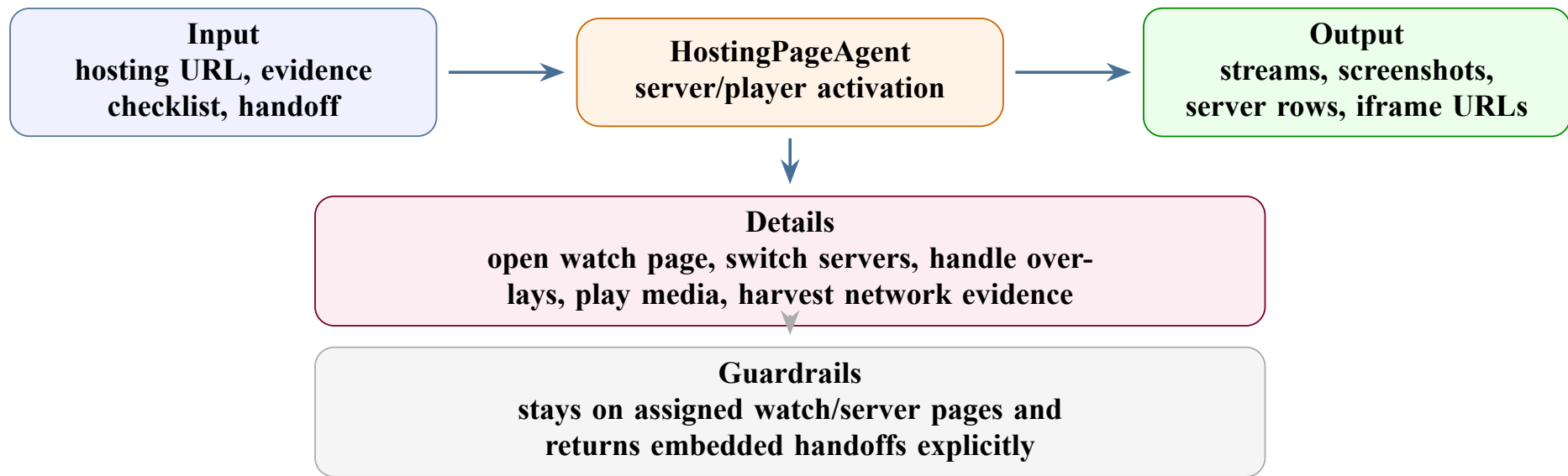
Figure 13: Hosting-page-agent design card.
