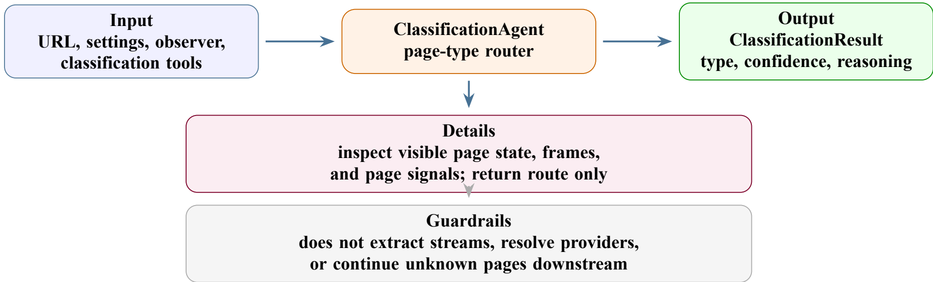
Figure 9: Classification-agent design card.
