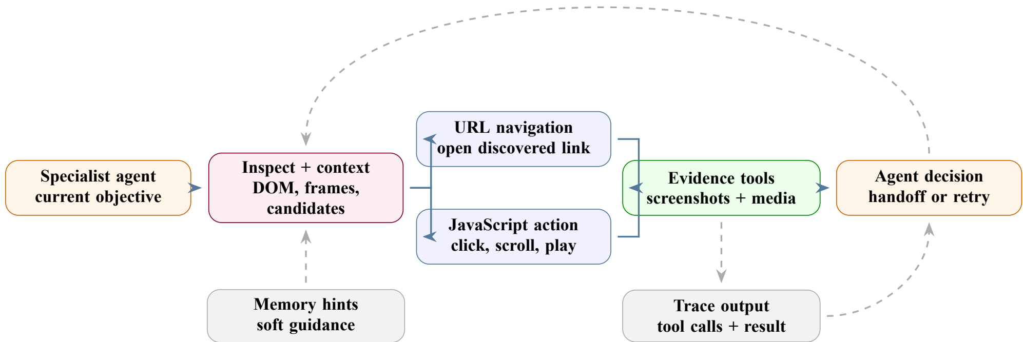
Figure 19: Global browser-tool flow: inspect first, choose URL navigation or JavaScript action, then validate evidence.
