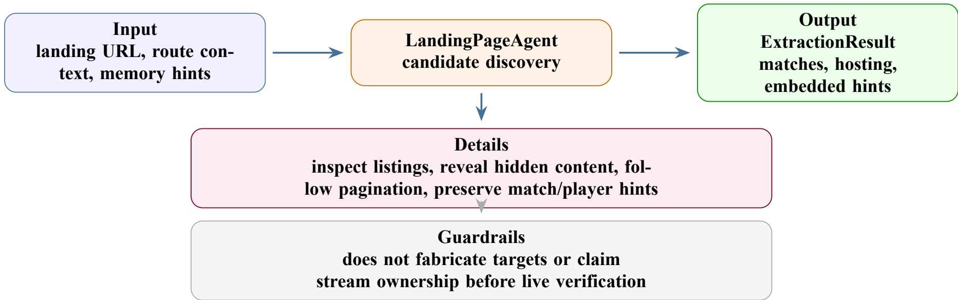
Figure 11: Landing-page-agent design card.
