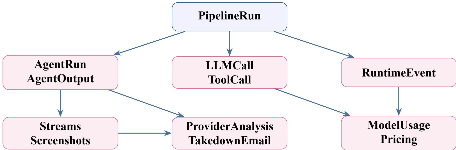
Figure 13: Simplified database relationship map for run review.
