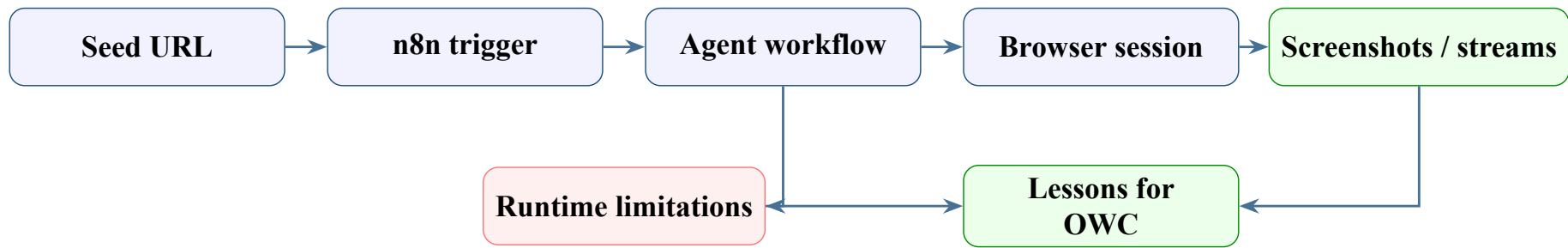
Figure 1: Role of the n8n workflow as a feasibility playground.
