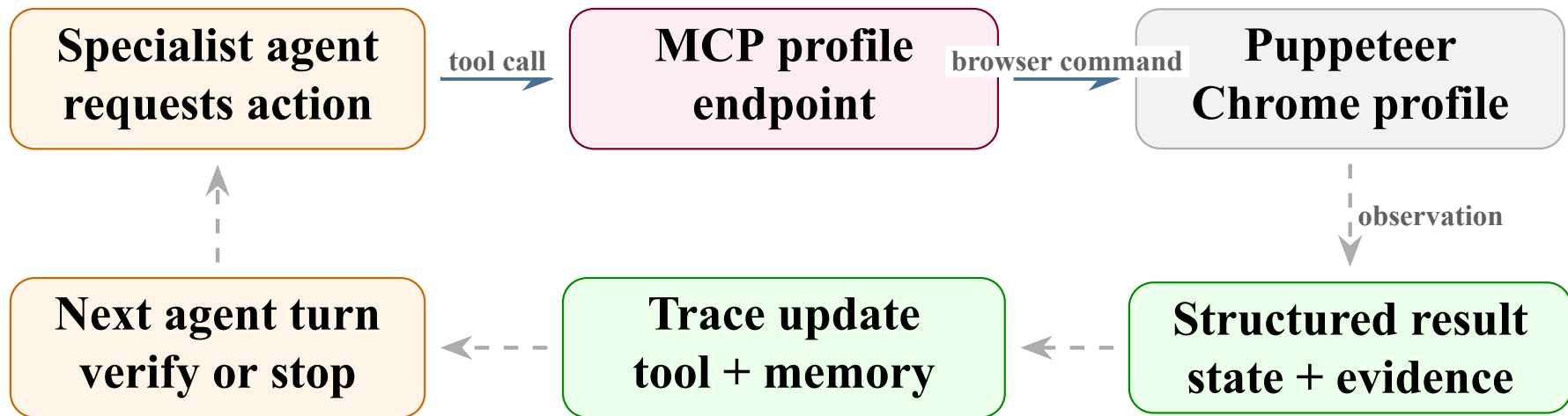
Figure 10: Browser tool execution loop through MCP and Puppeteer.
