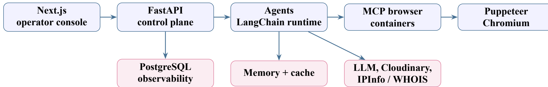
Figure 6: Five implementation areas of the Open Web Catcher platform.
