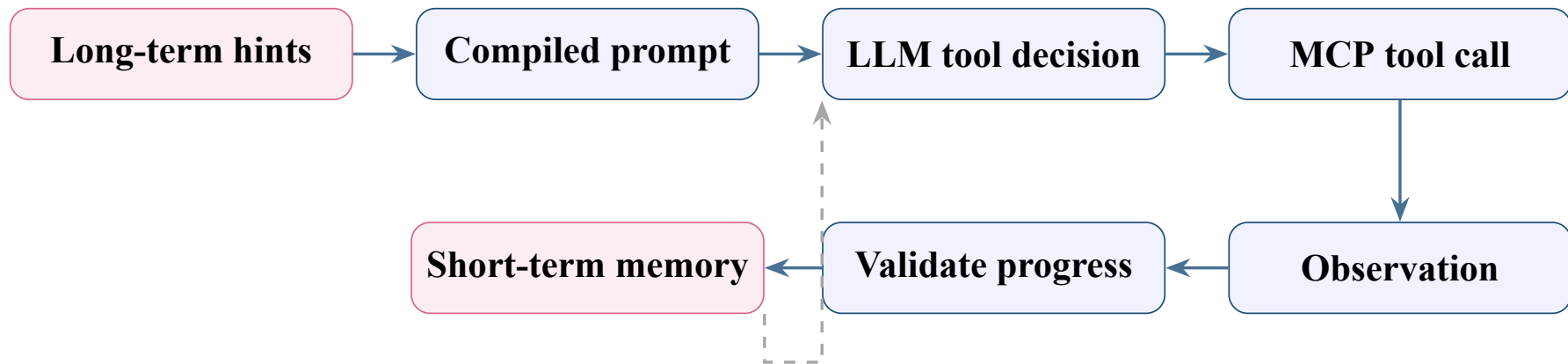
Figure 12: Agent reasoning loop with memory and tool feedback.
