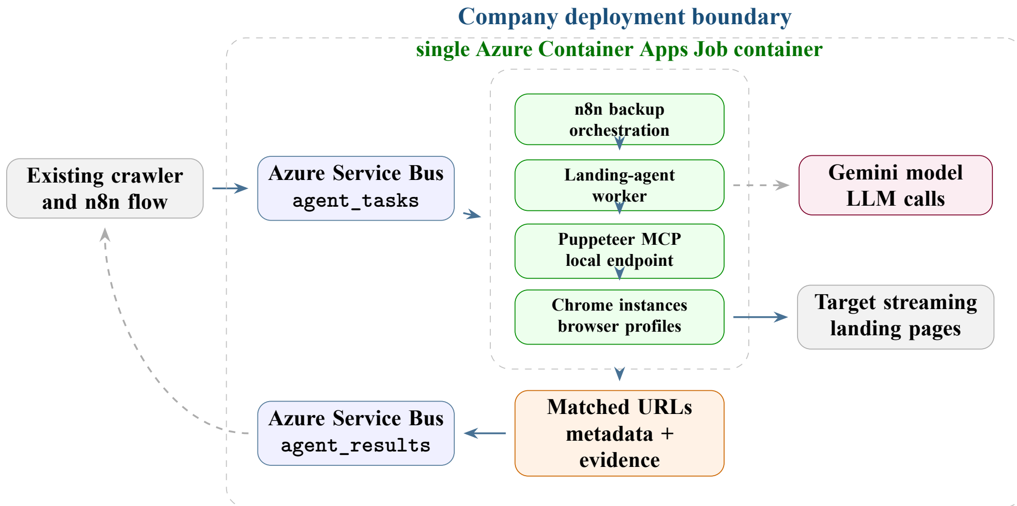
Figure 14: Company deployment flow using agent_tasks, a single n8n/Puppeteer landing-agent container, and agent_results.
