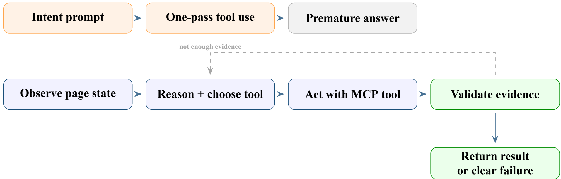
Figure 11: Prompt evolution from one-pass intent prompts to evidence-driven agent loops.
