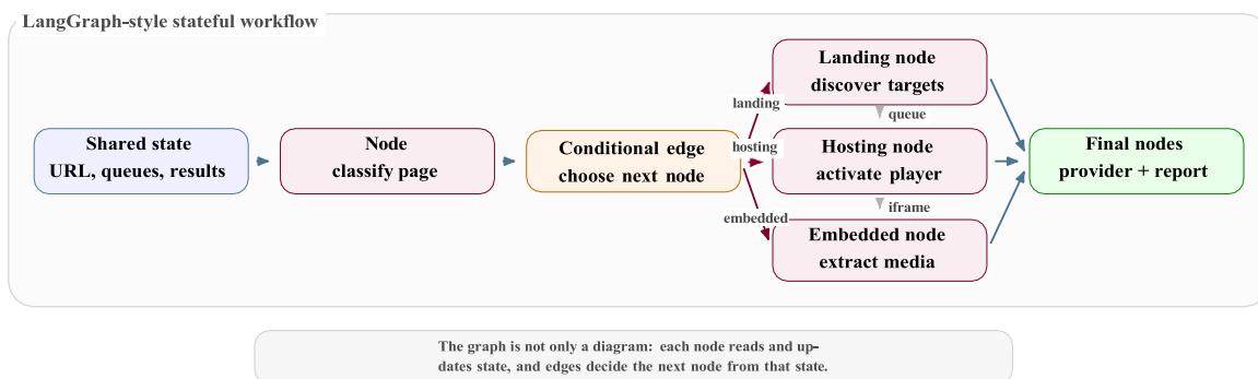
Figure 3.11: General LangGraph concept: named nodes, shared state, and conditional routing.
