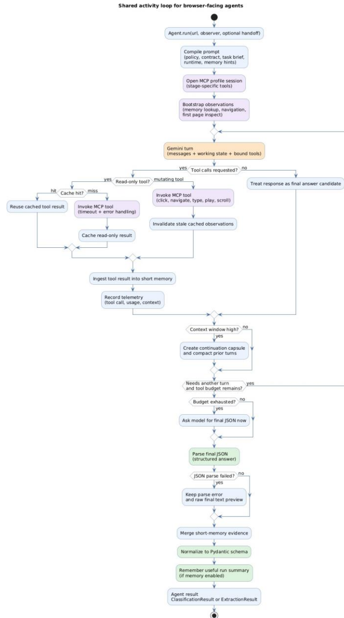
Figure 4.6: Shared activity loop for browser-facing agents.
