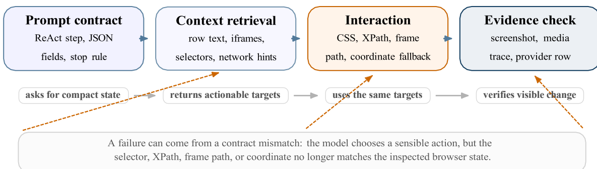
Figure 6.12: Prompt and tool-family alignment contract used during browser-agent evaluation.
