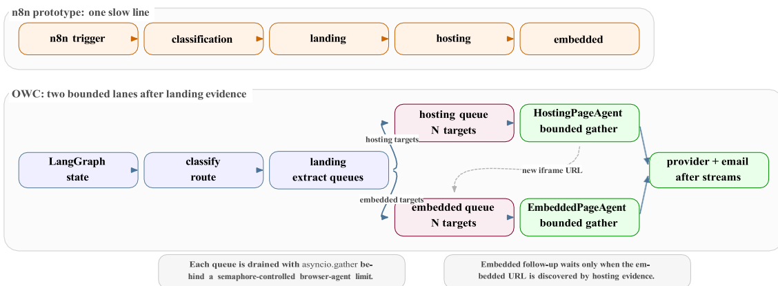
Figure 5.15: Sequential n8n execution compared with OWC’s LangGraph queues and bounded parallel agent execution.
