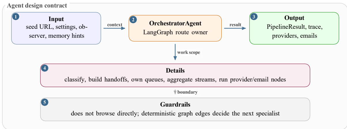
Figure 4.8: Orchestrator-agent design card.
