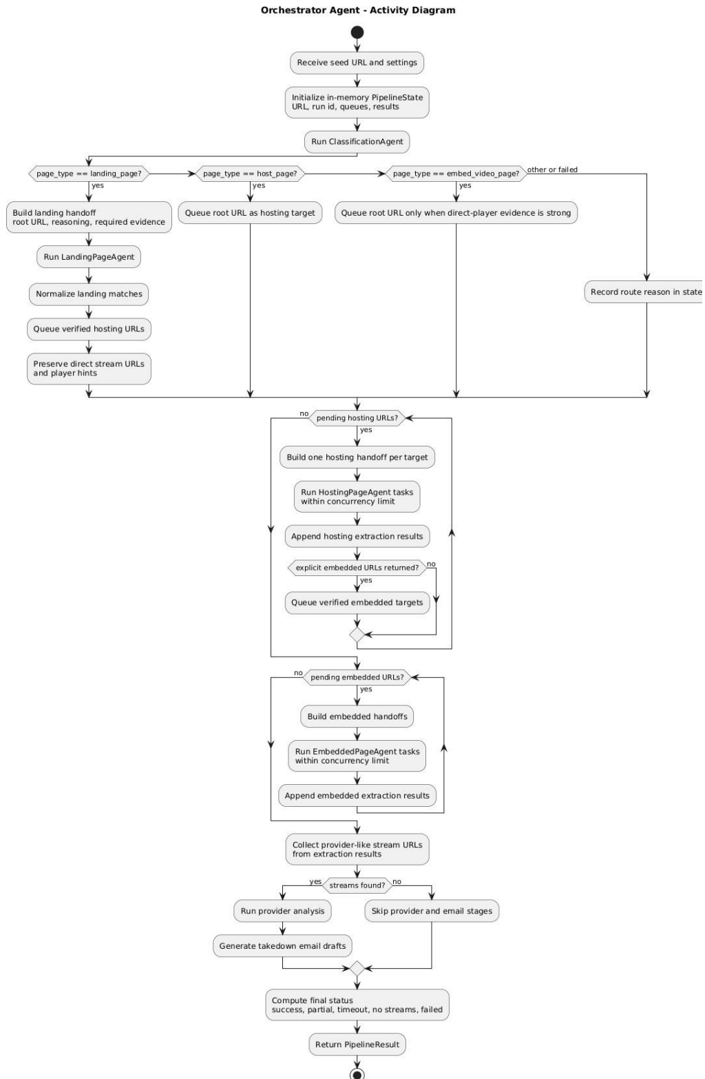
Figure 4.7: Orchestrator activity from run setup through classification, specialist routing, aggregation, provider/email handling, and final PipelineResult.
