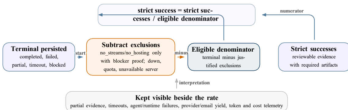
Figure 6.2: Strict-success denominator rule after external and no-evidence exclusions.
