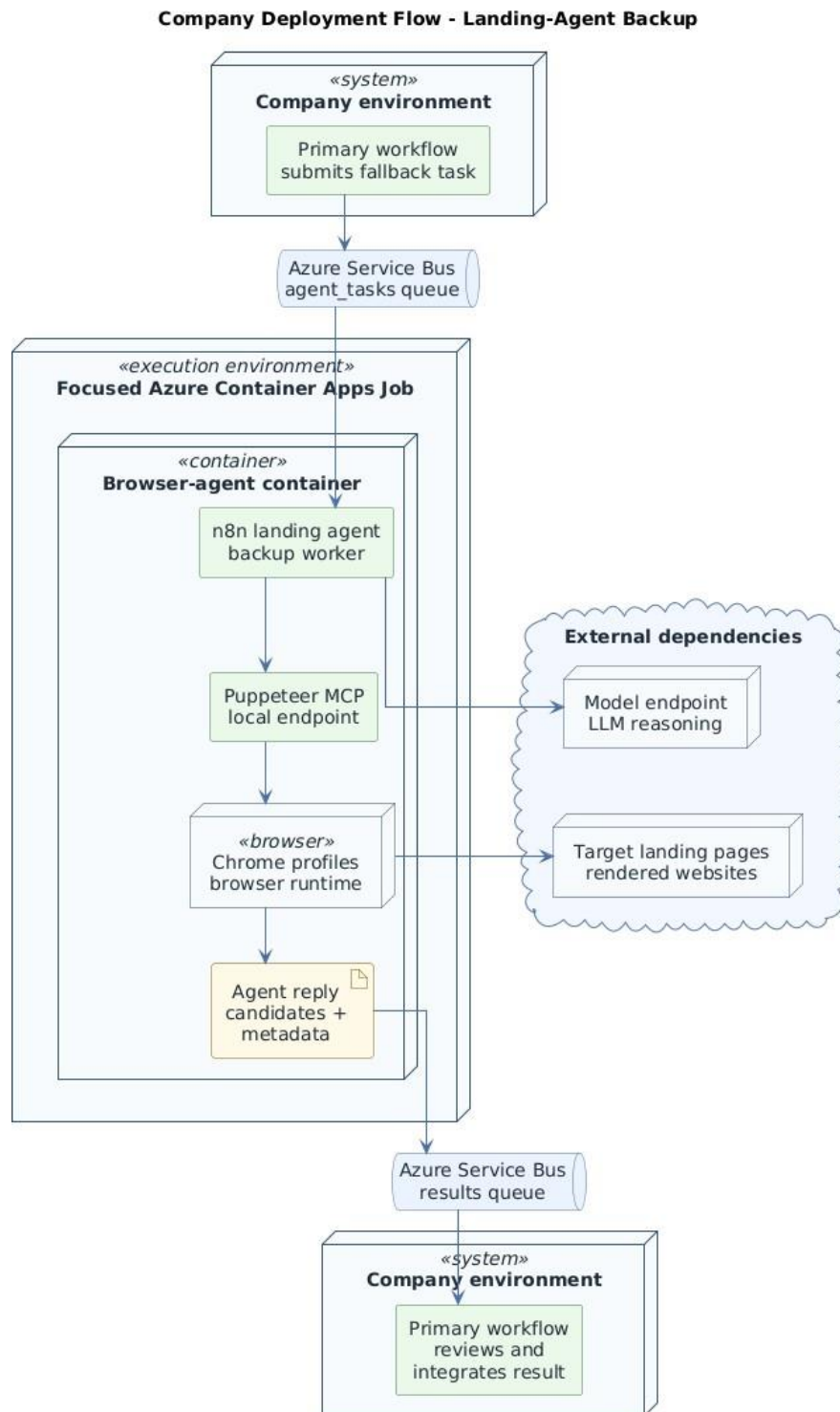
Figure 5.21: Company deployment flow for the landing-agent backup, from the primary workflow and Azure Service Bus queues to the focused Azure Container Apps job, browser runtime, external dependencies, and result payload.
