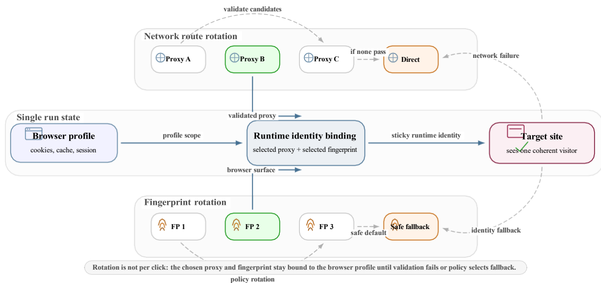
Figure 4.27: Proxy and fingerprint rotation as one coherent runtime identity.
