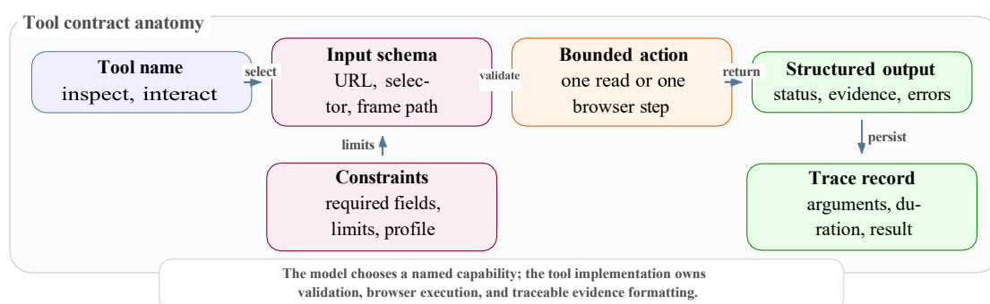
Figure 3.14: General structure of a tool contract used to connect an agent decision to executable browser code.
