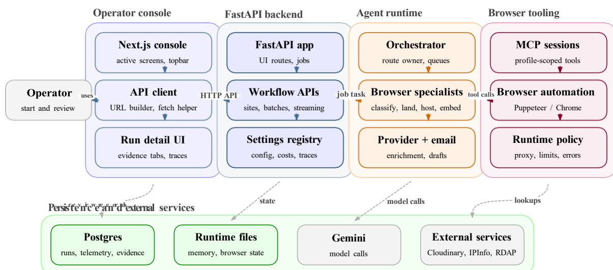
Figure 4.1: System component diagram for the OWC runtime.
