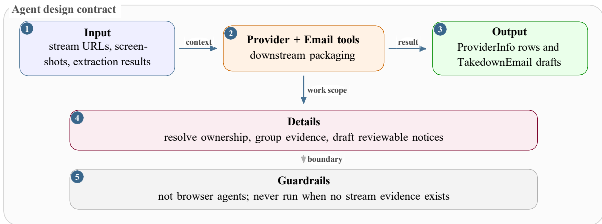
Figure 4.18: Provider-analysis and email-generation design card.
