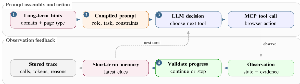
Figure 5.18: Agent reasoning loop with memory and tool feedback.
