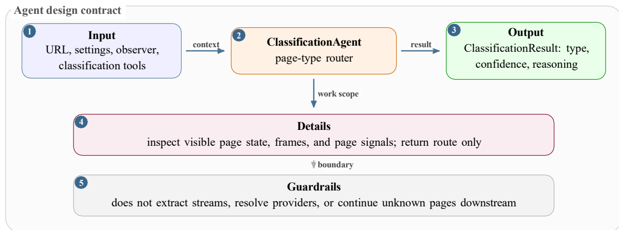
Figure 4.10: Classification-agent design card.
