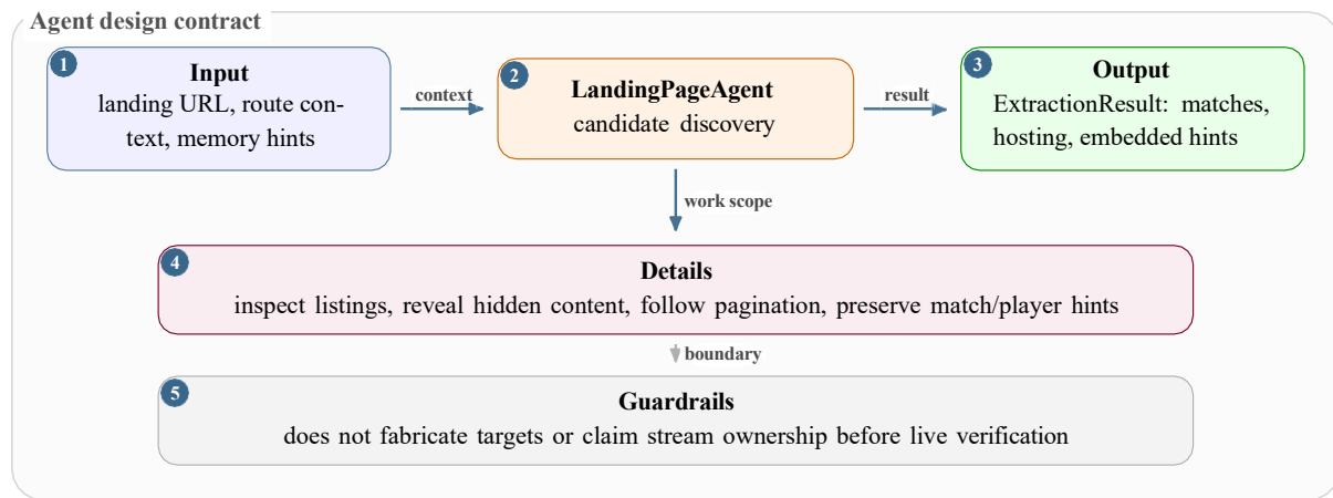
Figure 4.12: Landing-page-agent design card.
