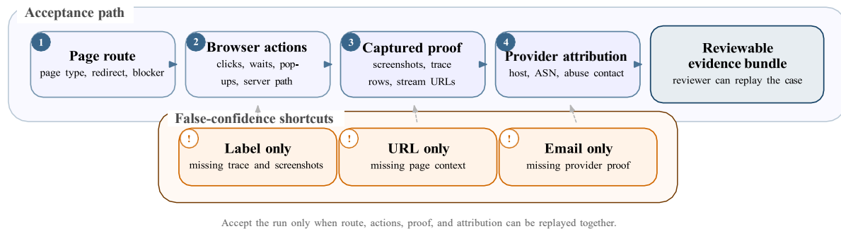
Figure 6.1: Evidence gate used to decide whether an OWC run is reviewable rather than merely labeled.
