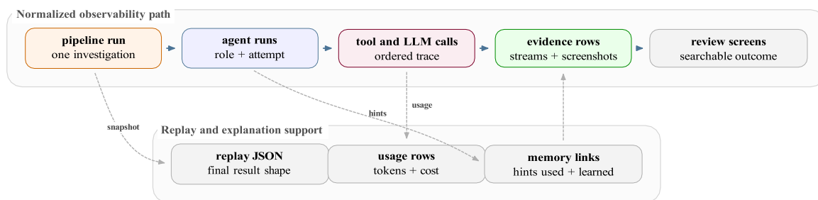
Figure 5.20: How PostgreSQL turns a parallel browser-agent run into replayable and searchable observability records.
