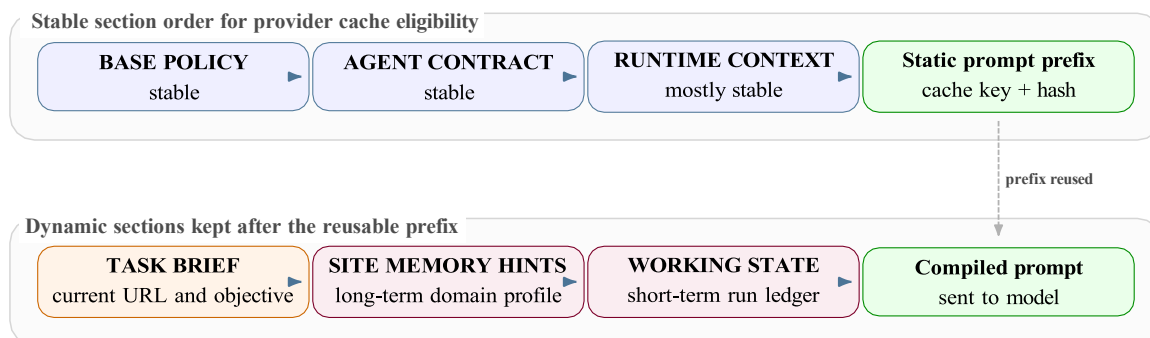
Figure 5.16: Prompt assembly layout used to keep stable instructions cache-eligible while memory and task state remain current.
