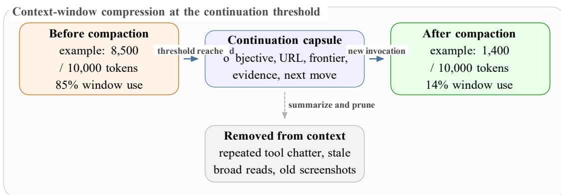
Figure 5.19: Before-and-after view of OWC context compaction when the model context approaches the configured threshold.
