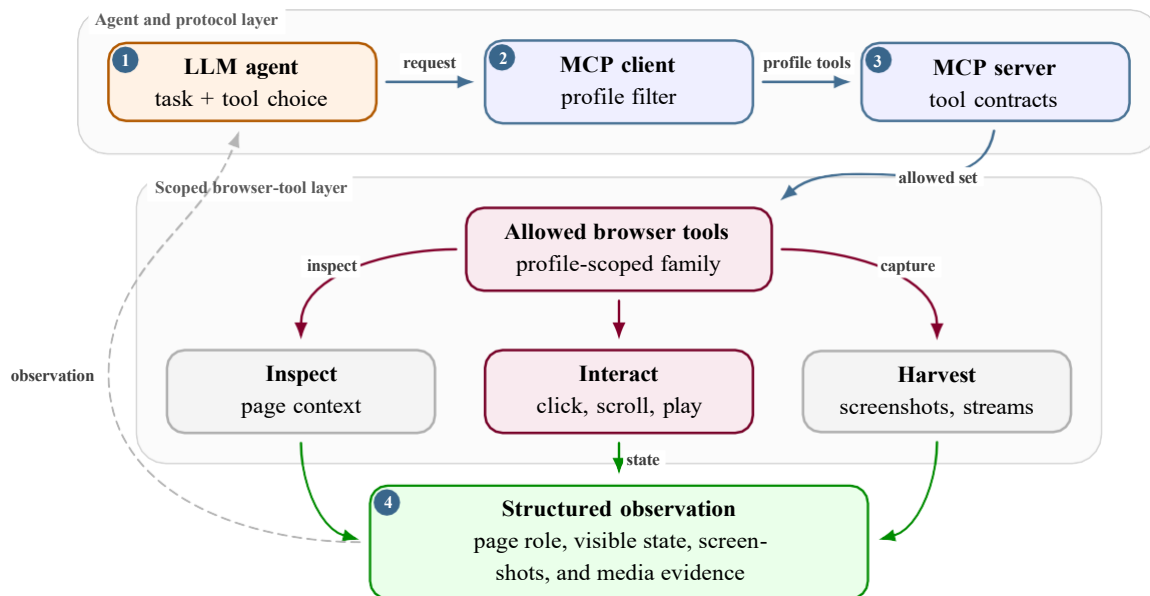
Figure 3.13: General MCP pattern connecting an LLM agent to scoped browser tools.
