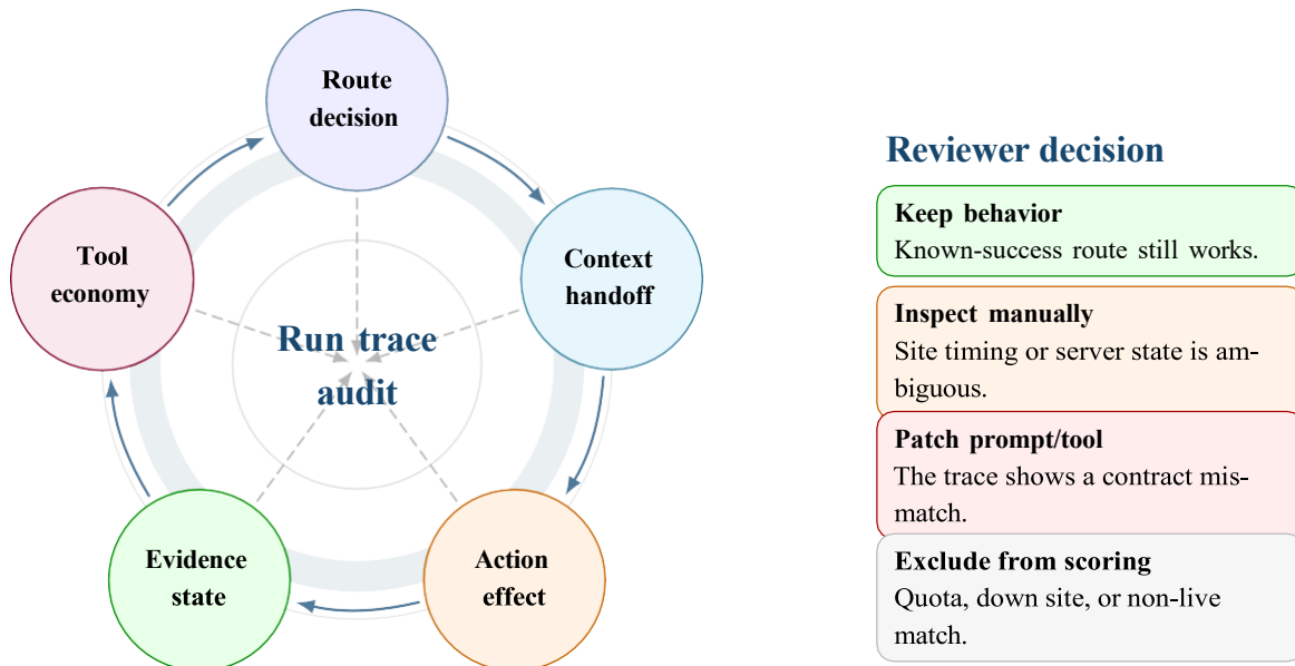
Figure 6.4: Trace-review loop used for agent evaluation. The reviewer separates route, context, action, evidence, and tool-economy signals before deciding whether a run proves agent quality, needs a prompt/tool patch, or should be excluded because the site or quota blocked the test.
