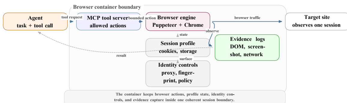
Figure 3.7: General browser-container concept used to isolate automated evidence collection.
