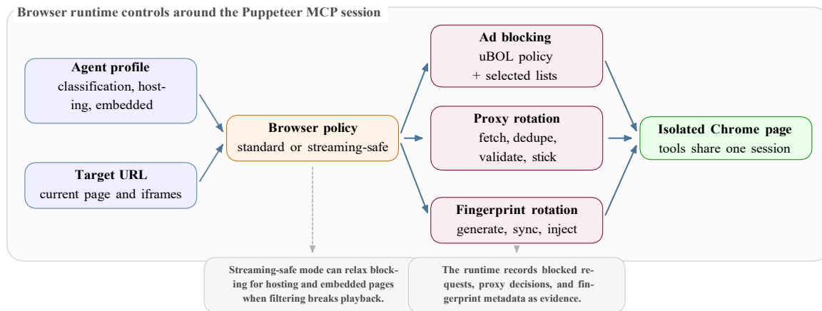
Figure 5.14: Runtime controls applied before a Puppeteer browser page is exposed to the MCP tools.
