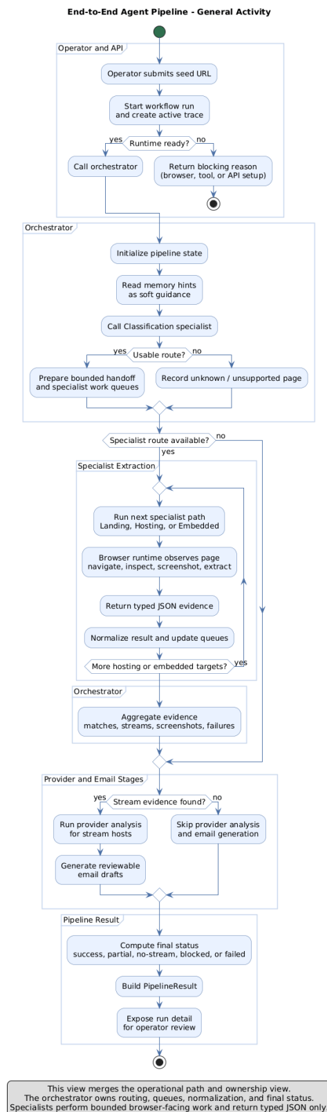
Figure 4.3: End-to-end agent pipeline as one activity diagram, from operator launch and runtime readiness through orchestrator routing, specialist extraction, provider analysis, email drafting, and the final PipelineResult.
