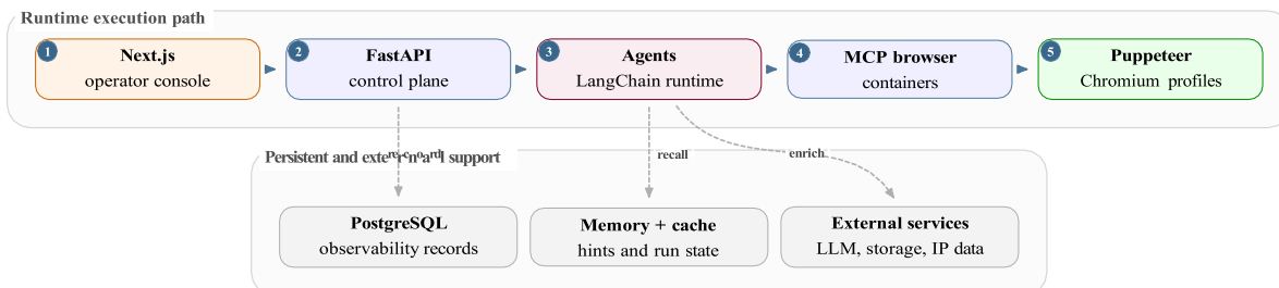
Figure 5.6: Five implementation areas of the Open Web Catcher platform.
