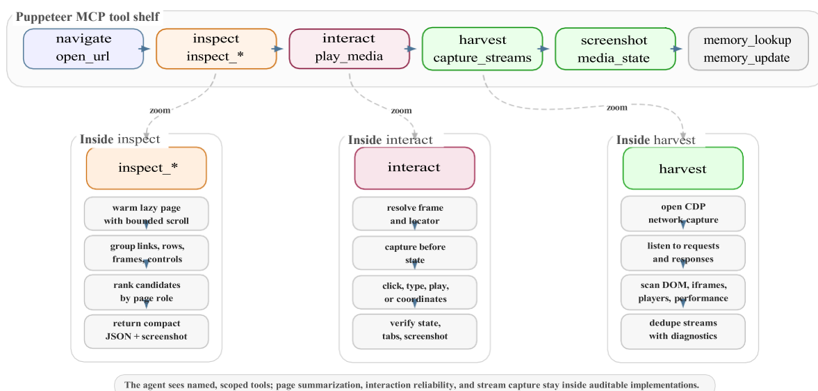
Figure 5.13: Puppeteer MCP toolbox with implementation zooms into inspect , interact , and harvest .
