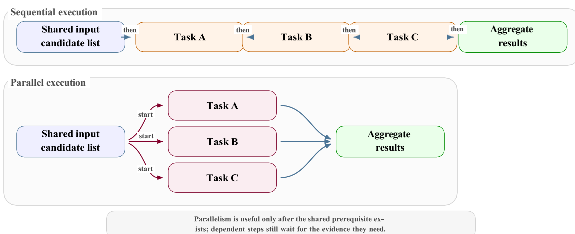
Figure 3.12: General difference between sequential and parallel workflow execution.
