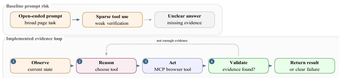
Figure 5.17: Prompt design contrast between an open-ended browser task and the evidence-driven agent loop used in OWC.
