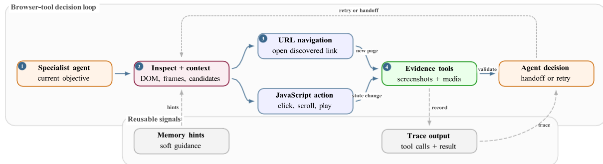
Figure 4.22: Global browser-tool flow.
