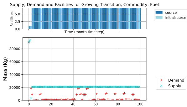
(b) Fuel demand and supply plot
