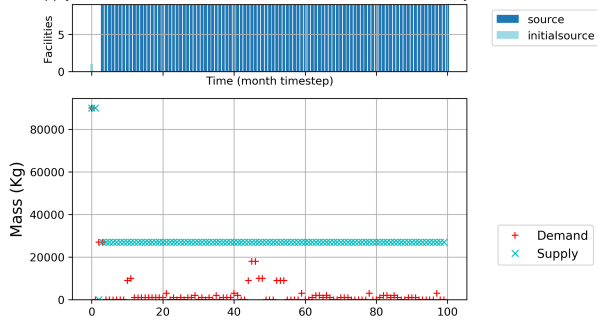
(b) Fuel demand and supply plot
