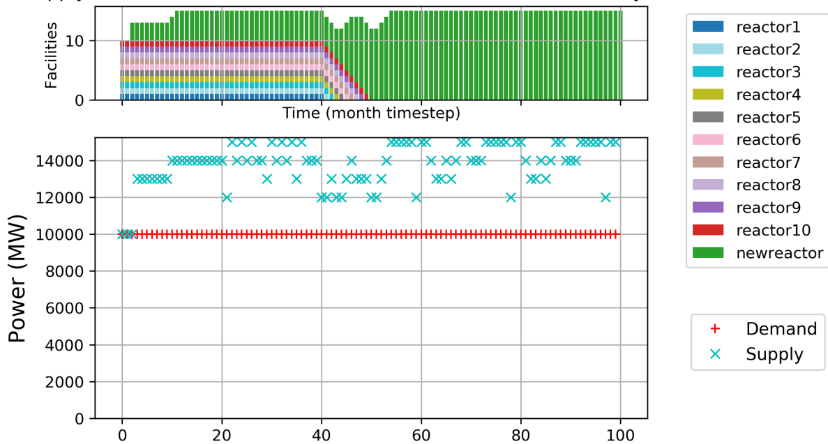
(a) Power demand and supply plot
