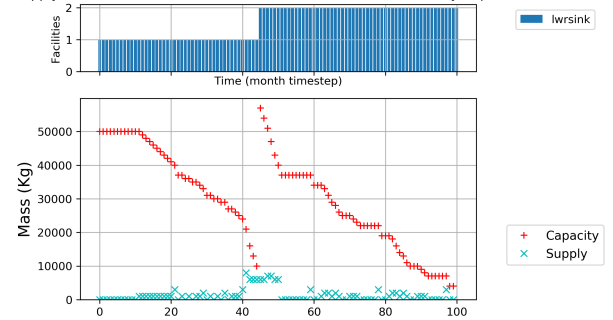
(c) Spent Fuel demand and supply plot
