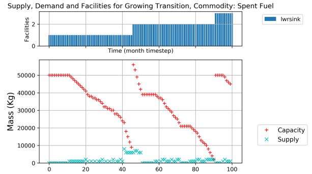
(c) Spent Fuel demand and supply plot
