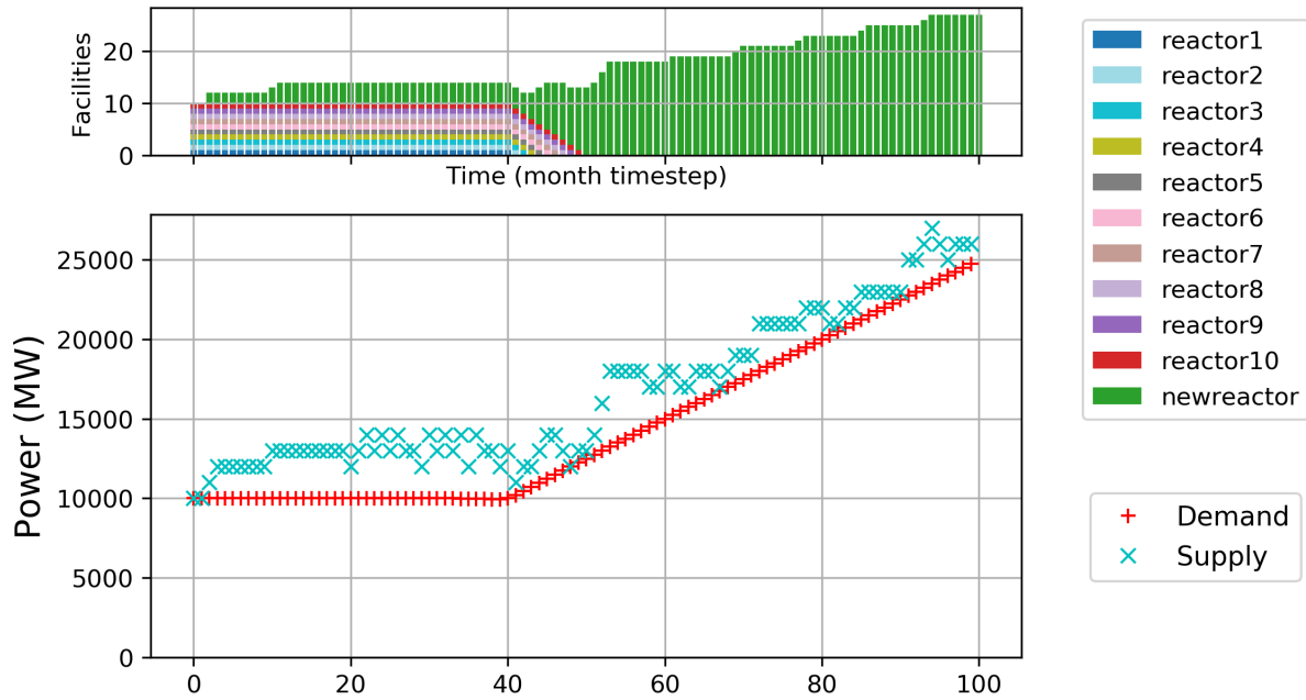
(a) Power demand and supply plot
