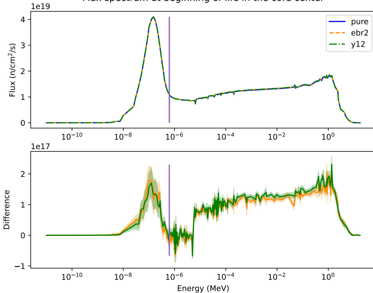
Flux spectrum at beginning of life in the core center
