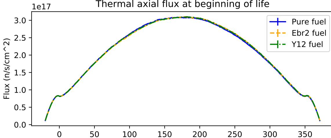
Thermal axial flux at beginning of life
