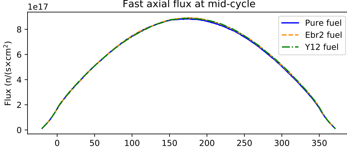
Fast axial flux at mid-cycle
