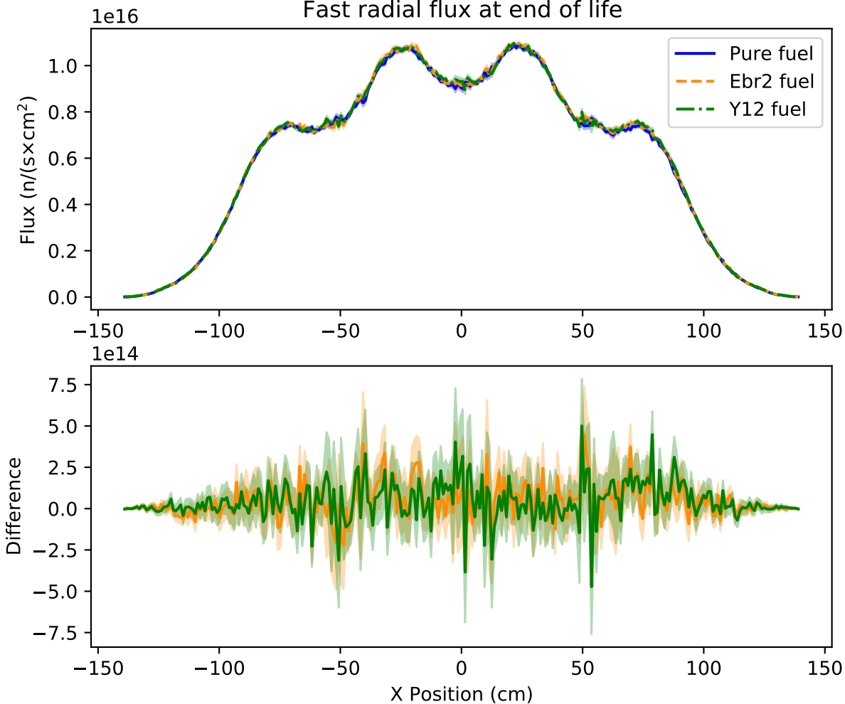
Fast radial flux at end of life
