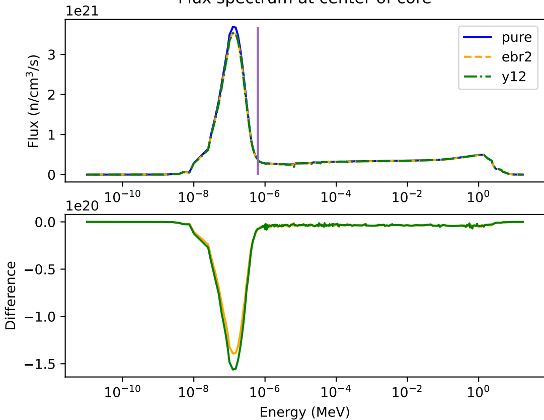
Flux spectrum at center of core
