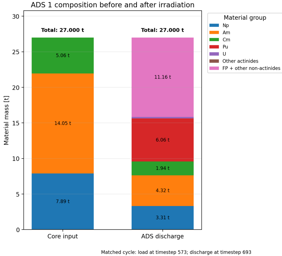
Figure 4.13: Stacked comparison of the material entering and leaving one representative ADS 1 irradiation cycle. The 27 t input contains neptunium, americium, and curium. The discharge contains approximately 15.84 t of remaining actinides and 11.16 t of fission products and other non-actinides. The net actinide reduction is approximately 11.16 t, or 41.3% of the input actinide mass. Plutonium and the small uranium component in the discharge are descendant actinides produced during irradiation.
