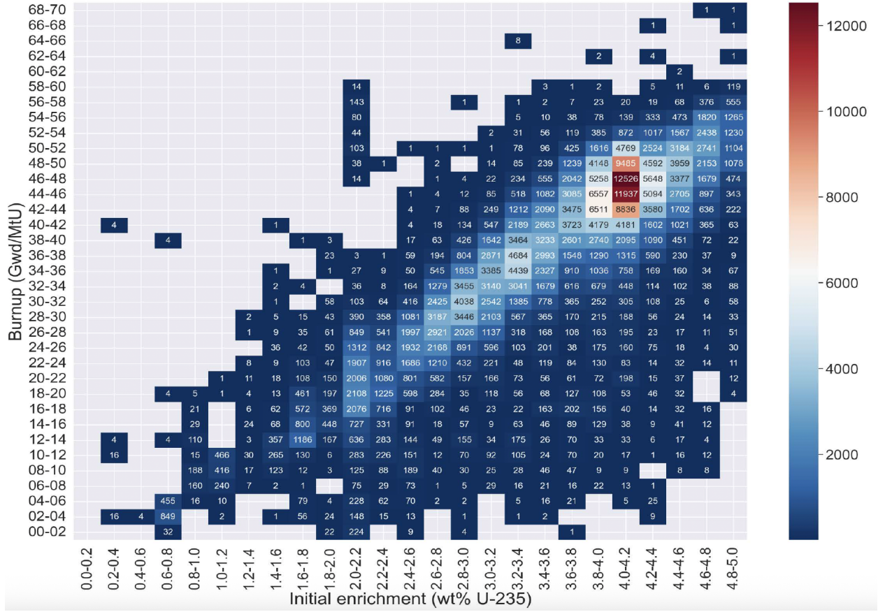
Figure 2.2: Burnup (GWd/MTHM) and initial enrichment (% ^{235}\text{U} ) distributions for spent nuclear fuel assemblies in the LWR inventory through December 2022. The color scale and the value in each cell indicate the number of assemblies in the corresponding burnup–enrichment bin. Figure reproduced from [2].
