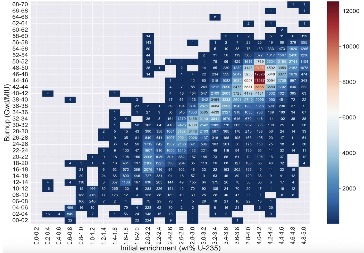
Figure 2.2: Burnup (GWd/MTHM) and initial enrichment (% ^{235}\text{U} ) distributions for spent nuclear fuel assemblies in the LWRs inventory through December 2022 [2].
