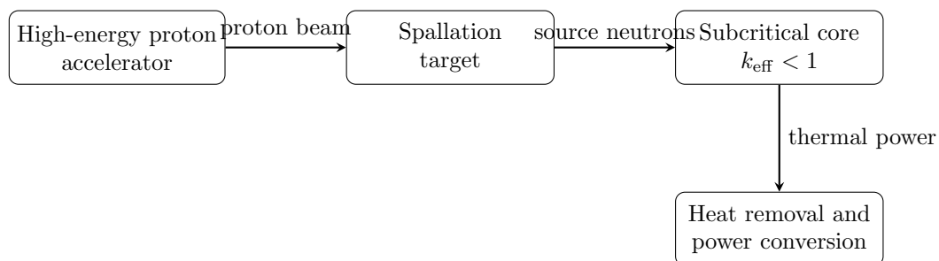
Figure 2.4: Principal components and energy flows of an accelerator-driven subcritical system. This original schematic is based on the ADS descriptions presented in [20,21].
