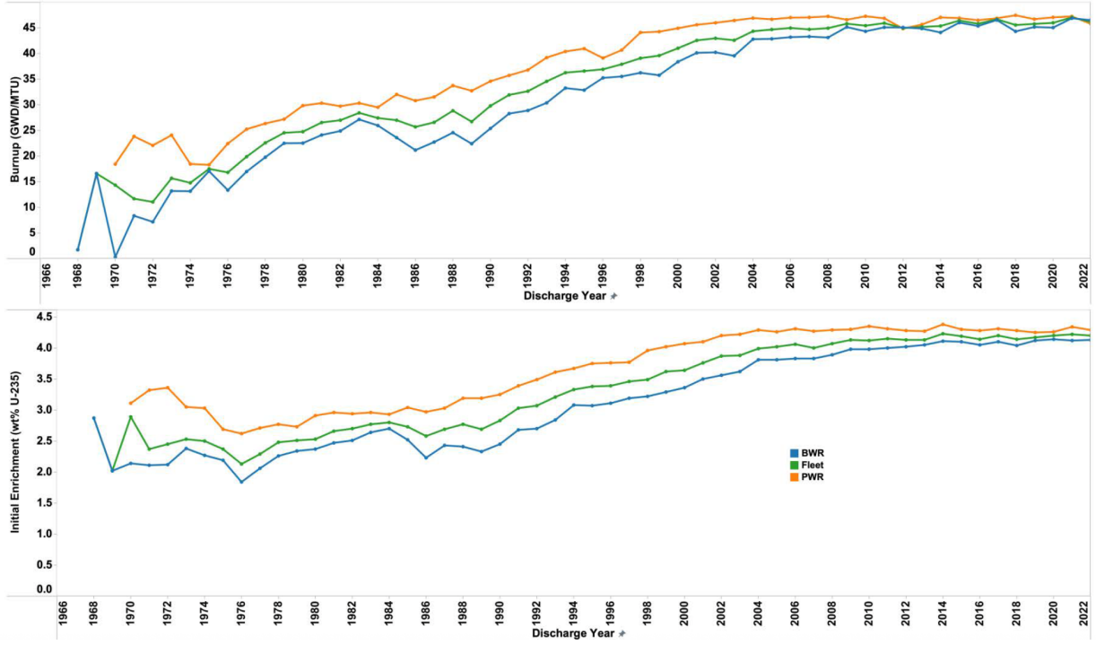
Figure 2.1: The annual average discharge burnup and initial ^{235}\text{U} enrichment of U.S. light-water-reactor fuel increased substantially between 1968 and 2022 [2].
