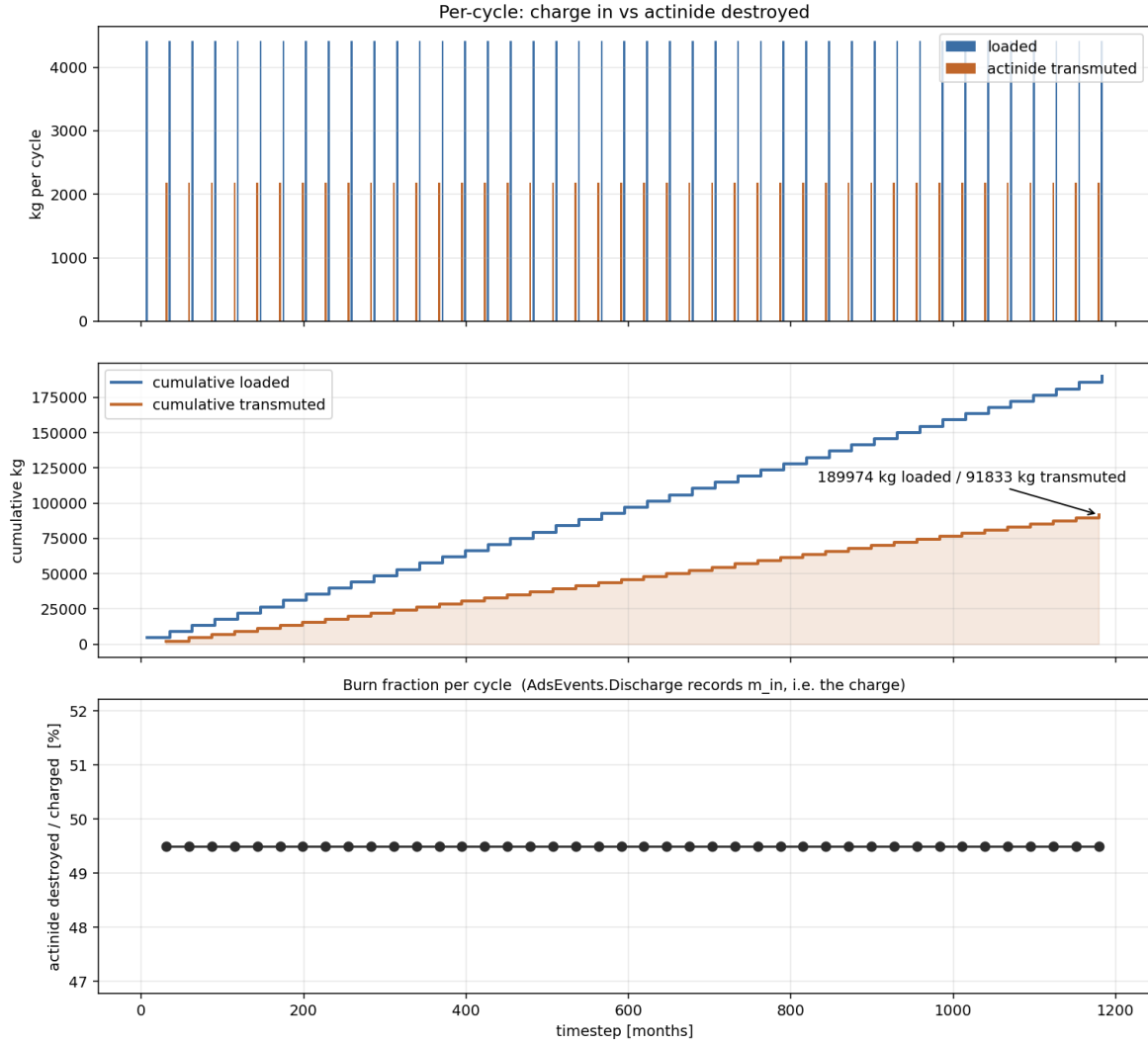
Figure 4.7: Per-cycle charge and actinide destruction for the 50/50 plutonium-minor-actinide core (ADS 2), 100-year recycling run. Each cycle charges 4.4 t and records 2.2 t of net actinide destruction, a burn fraction just under 50%. The small, fast-cycling core completes 42 cycles over the horizon.
