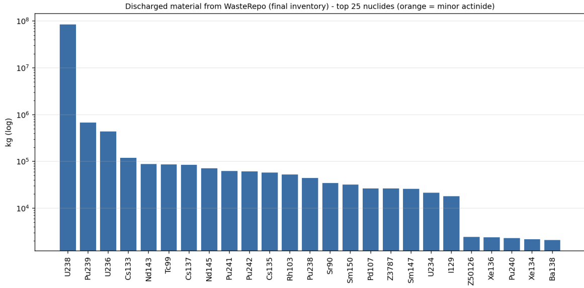
Figure 4.11: Final waste-repository composition for the minor-actinide-only recycling run (ADS 1), showing the 25 most abundant nuclides on a logarithmic mass scale; minor actinides are highlighted. The stream is dominated by uranium and plutonium stripped by separations, while minor actinides are nearly absent, having been recovered and burned.
