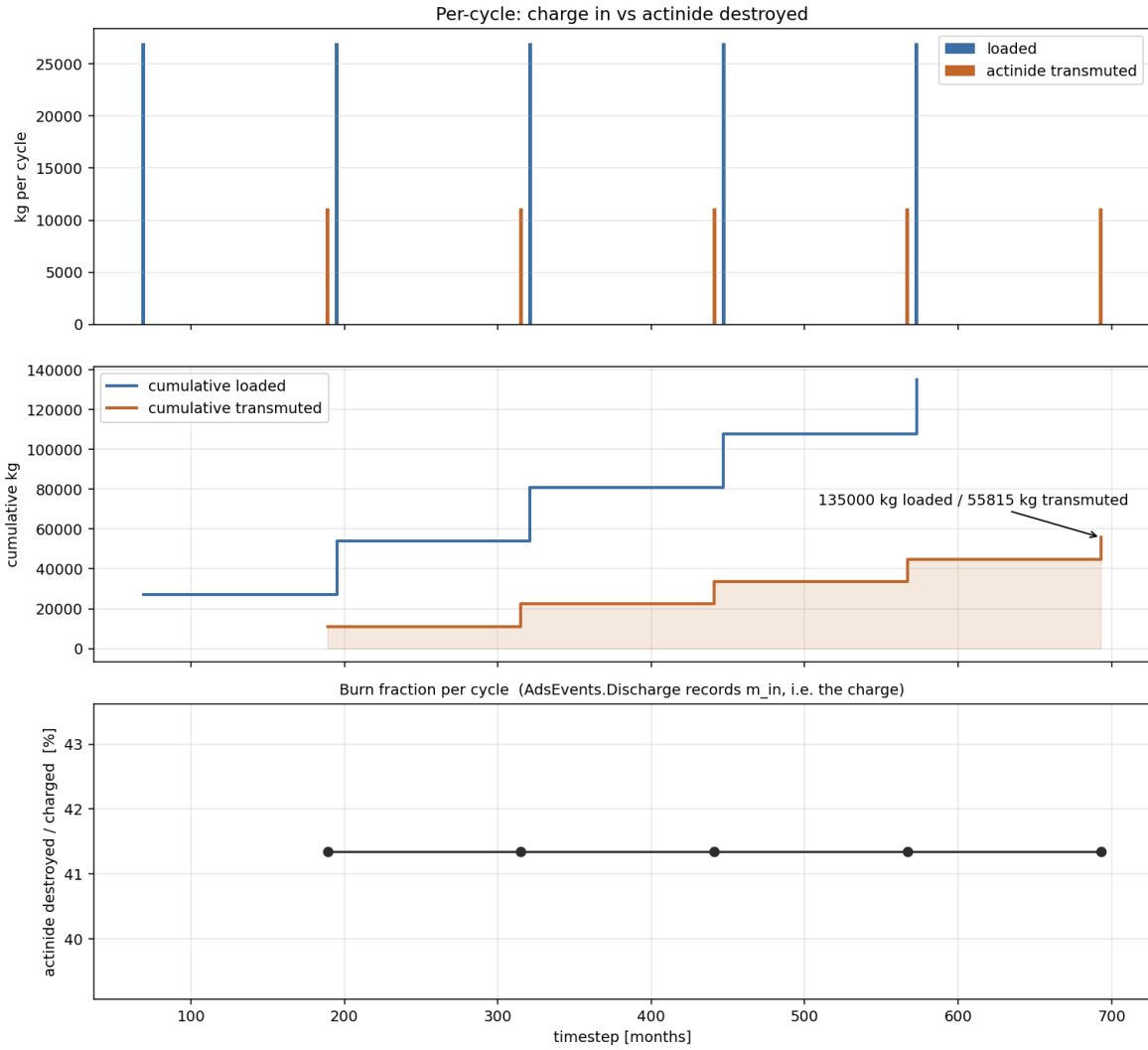
Figure 4.6: Per-cycle charge and actinide destruction for the minor-actinide-only core (ADS 1), 100-year recycling run. Each cycle charges 27 t and records 11.15 t of net actinide destruction, a constant burn fraction of 41.3% (bottom panel). The cumulative panel (centre) reaches 135 t charged and 55.8 t of cumulative net actinide destruction over five cycles.
