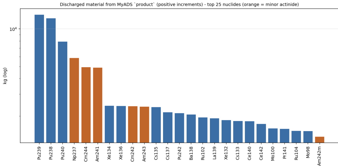
Figure 4.12: Composition of the material discharged from the ADS in the 50/50 recycling run (ADS 2), showing the 25 most abundant nuclides on a logarithmic mass scale; minor actinides are highlighted. Plutonium leads the recovered stream, followed by the minor actinides and fission products, all of which recycling returns to the feed.
