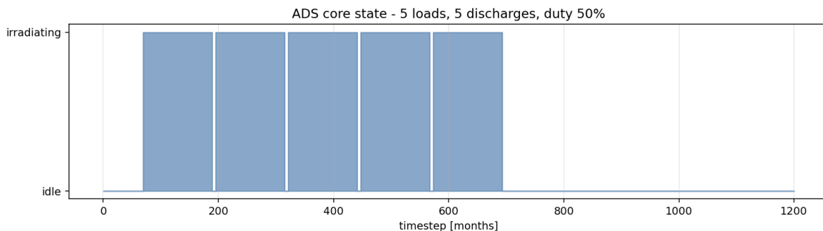
Figure 4.8: Irradiating-or-idle state of the minor-actinide-only core (ADS 1) over the 100-year recycling run. The core completes five ten-year cycles and then falls idle because its recoverable Np-Am-Cm feed no longer reaches the 27 t full-core loading threshold; the duty factor is 50%.
