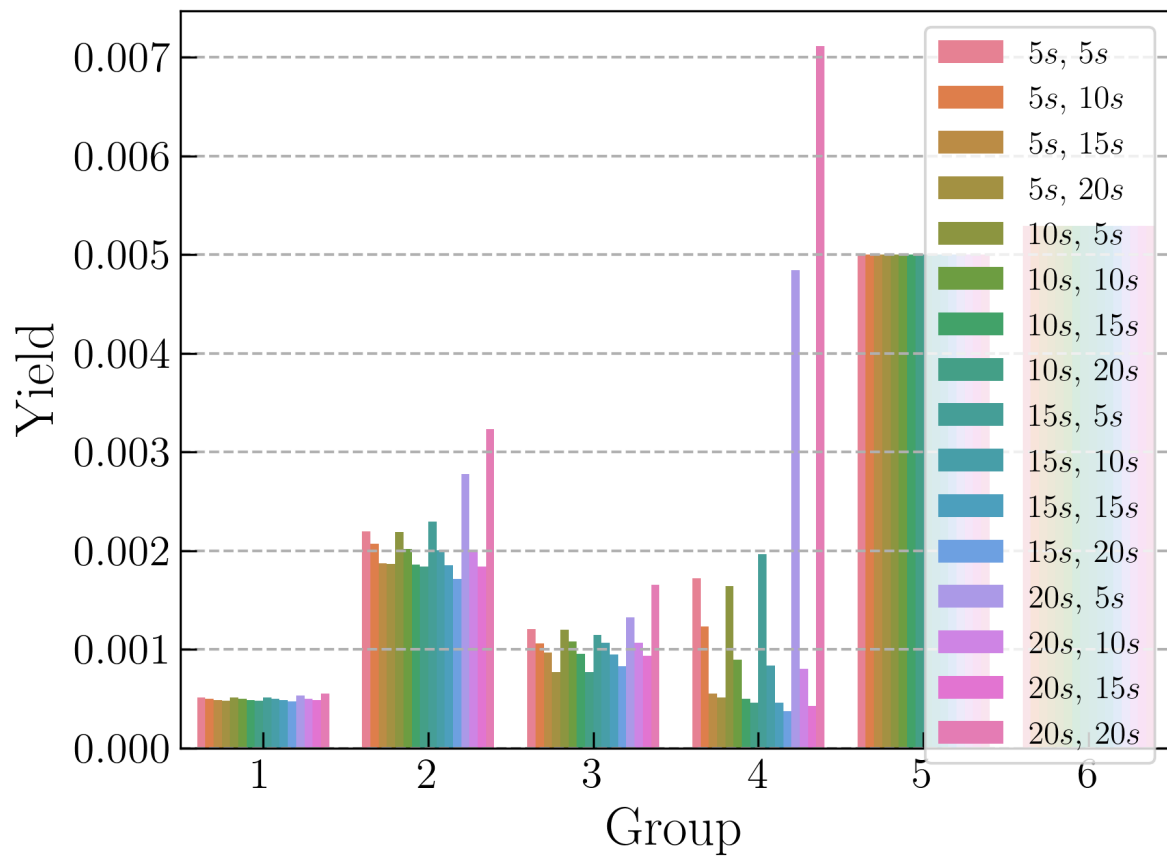
Figure 4.10: Group yields for various residence times during irradiation in OpenMC.
