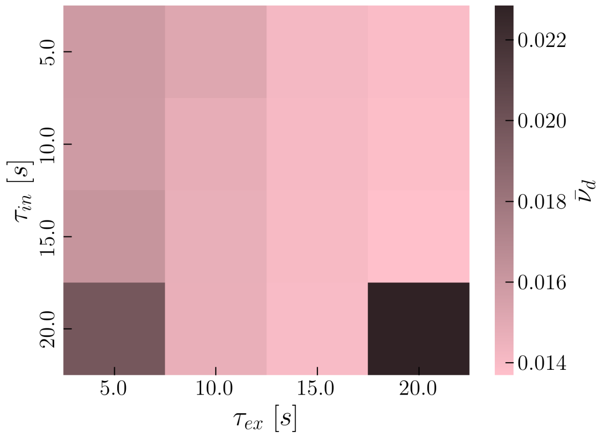
Figure 4.9: Total delayed neutron yield for various residence times during irradiation in OpenMC.
