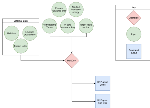
Figure 6: Flow diagram of 0D scaled model used to generate improved DNP group parameters.
