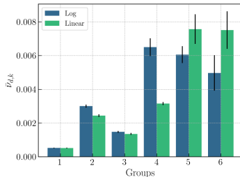
Figure 13: \bar{\nu}_{d,k} for each DNP group k after a thermal saturation irradiation of ^{235}\text{U} using the 0D scaled model.
