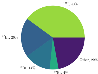
Figure 6: Relative delayed neutron counts from each DNP after a thermal saturation irradiation of ^{235}\text{U} using the 0D scaled model.
