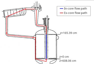
Figure 3: The flow path and bounds for the in-core region of the MSRE, overlayed on the MSRE loop diagram from [10].
