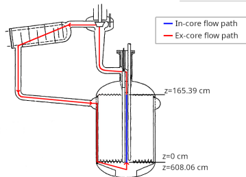
Figure 1: The flow path and bounds for the in-core region of the MSRE, overlaid on the MSRE loop diagram from [10].
