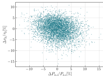
Figure 21: DNP group 3 half-life variation due to ^{87}\text{Br} emission probability variation with a PCC of -0.19.
