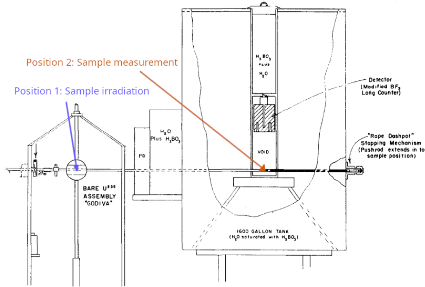
Figure 2.1: Simplified experimental setup for measuring delayed neutron emission from irradiation of a 3 gram sample in Godiva referenced from [90].
