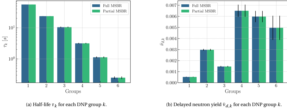
Figure 4.3: Delayed neutron contributions from each DNP with and without long cycle time chemical removal rates in the MSBR after a thermal saturation irradiation of ^{235}\text{U} using the 0D scaled model. The differences induced by exclusion of removal rates with cycle times longer than 20 seconds are minimal and well within uncertainty bounds.
