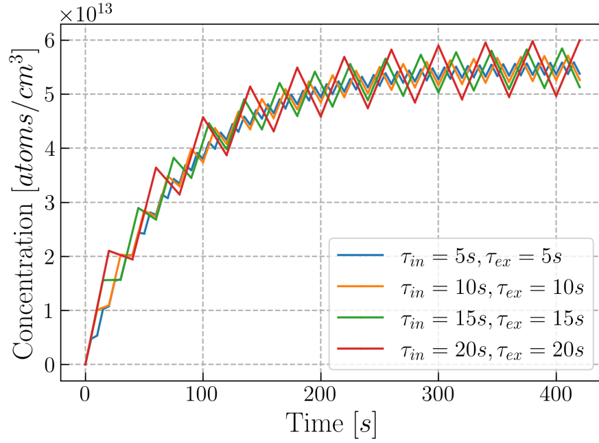
Figure 4.9: A comparison of various in-core and ex-core residence times on the concentration of ^{87}\text{Br} during irradiation of the sample over 420 seconds.
