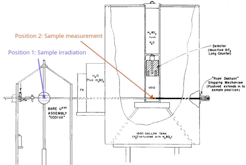
Figure 2.1: Simplified experimental setup for measuring delayed neutron emission from irradiation of a 3 gram sample in Godiva referenced from [79].
