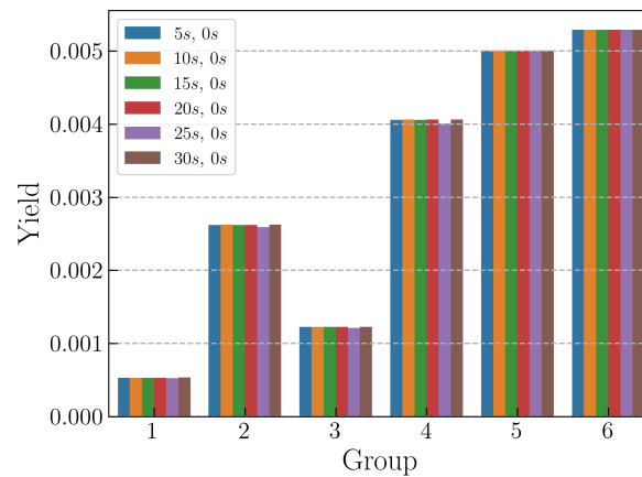
Figure 4.10: Group yields for a static irradiation in OpenMC with varying in-core residence times.
