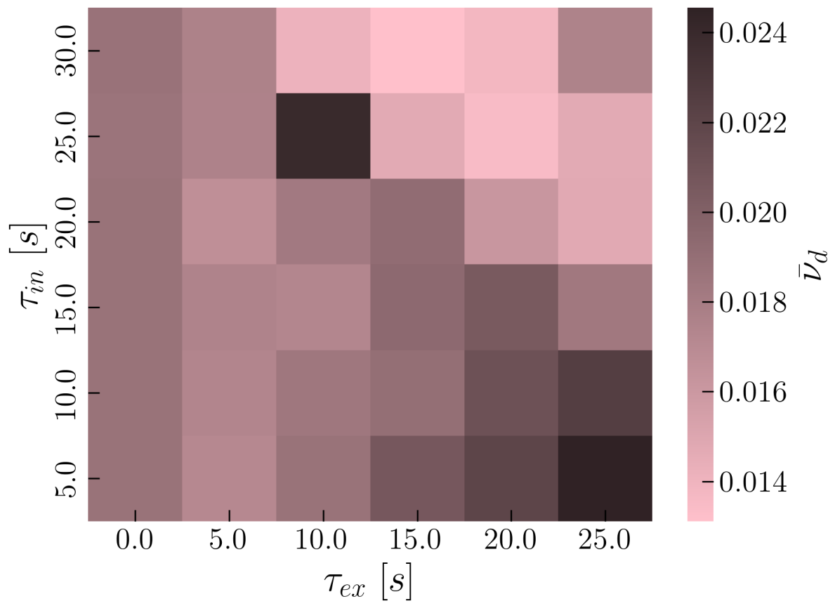
Figure 4.11: Total delayed neutron yield for various residence times during irradiation in OpenMC.
