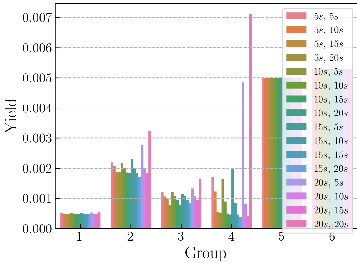
Figure 4.12: Group yields for various residence times during irradiation in OpenMC.
