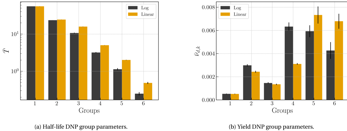
Figure 4.5: DNP group parameters for linear and logarithmic spacings of the time nodes.
