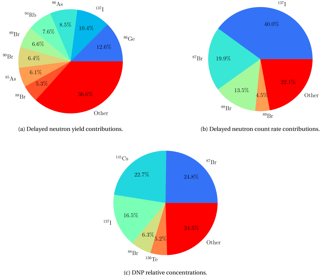
Figure 4.1: Delayed neutron contributions from each DNP.
