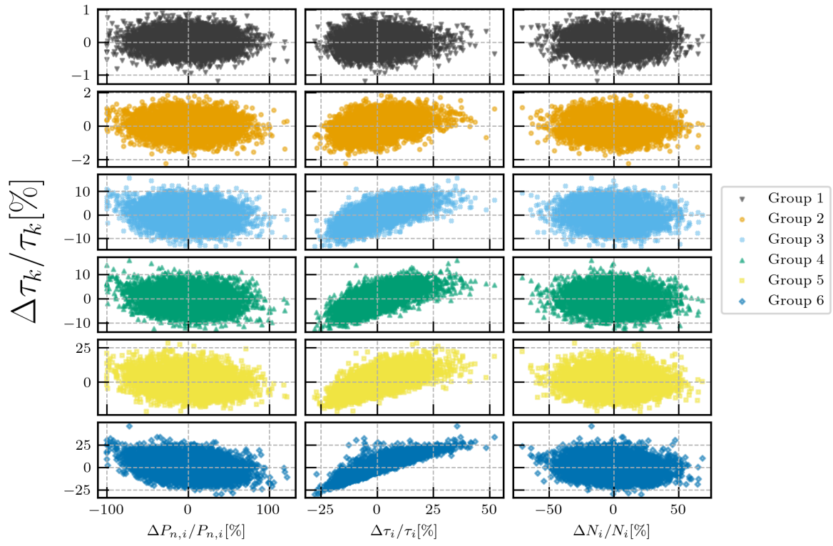
Figure 4.12: The difference in each DNP group half-life from the ^{86}\text{Ge} relative changes in emission probability, half-life, and concentration.
