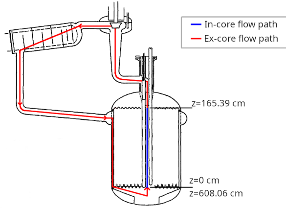
Figure 3.2: The flow path and bounds for the in-core region of the MSRE, overlayed on the MSRE loop diagram from [53].
