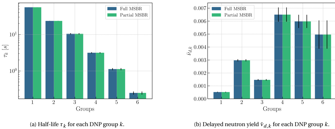
Figure 4.3: Delayed neutron group parameters calculated with and without long cycle time chemical removal rates in the MSBR after a thermal saturation irradiation of ^{235}\text{U} using the 0D scaled model. The differences induced by exclusion of removal rates with cycle times longer than 20 seconds are minimal and well within uncertainty bounds.
