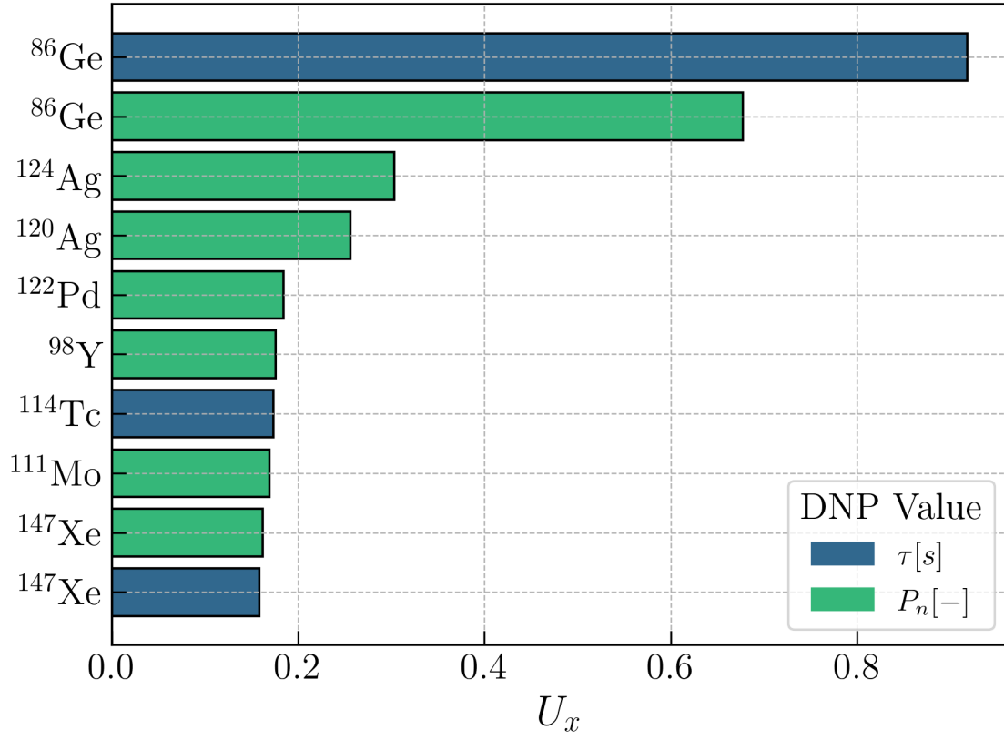
Figure 4.16: The sum of the PCC magnitudes times the relative uncertainties for each DNP, isolated by DNP value x , on each group half-life \tau_k and yield \bar{v}_{d,k} after a thermal saturation irradiation of ^{235}\text{U} using the 0D scaled model. The ^{86}\text{Ge} values are noticeably larger, and the most important data to improve are the half-lives and emission probabilities for short-lived DNP.
