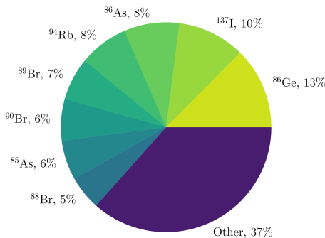
Figure 5: Relative delayed neutron yield from each DNP after a thermal saturation irradiation of ^{235}\text{U} using the 0D scaled model.
