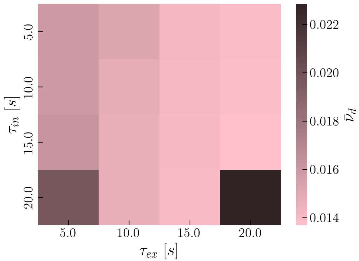
Figure 4.10: Total delayed neutron yield for various residence times during irradiation in OpenMC.
