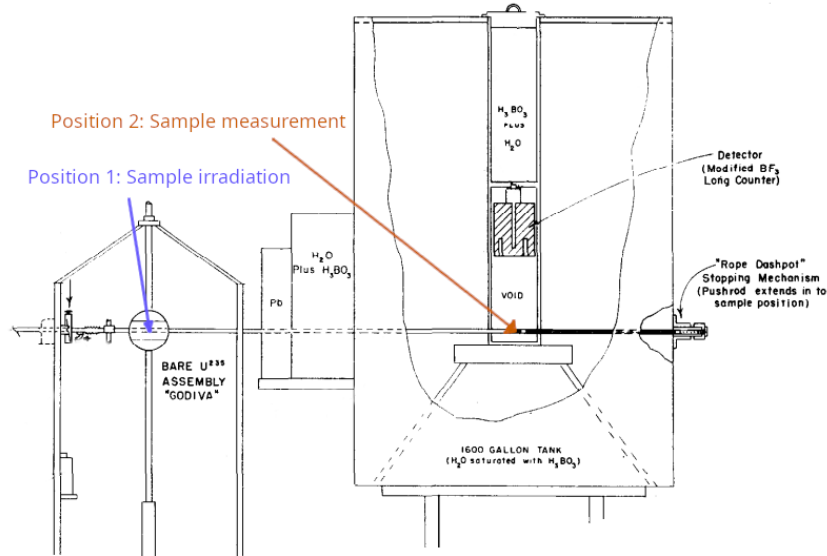
Figure 2.1: Simplified experimental setup for measuring delayed neutron emission from irradiation of a 3 gram sample in Godiva referenced from [76].
