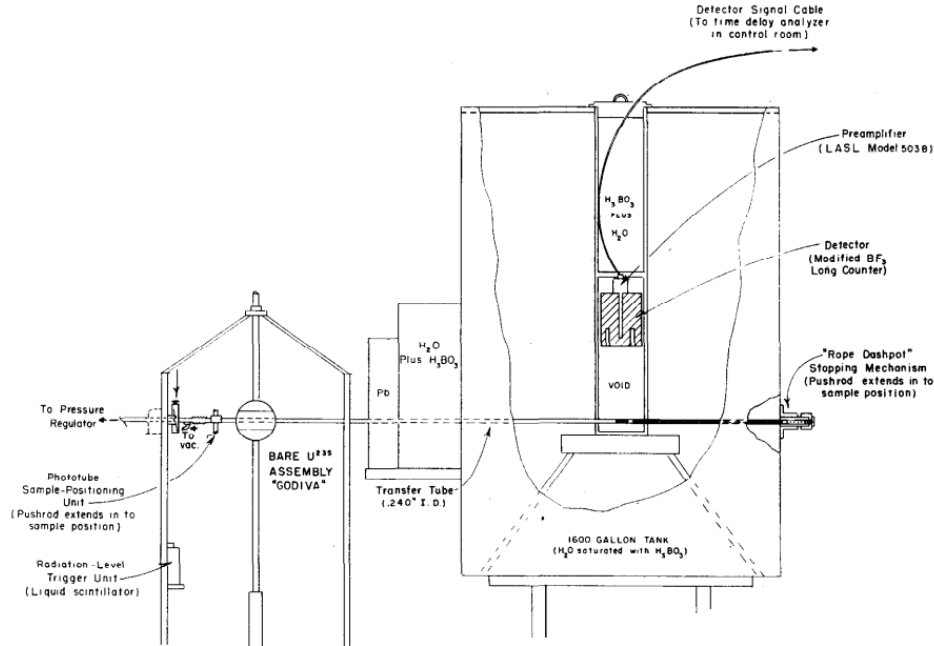
Figure 2.1: Experimental setup for measuring delayed neutron emission from irradiation of a 3 gram sample in Godiva recreated from [66].
