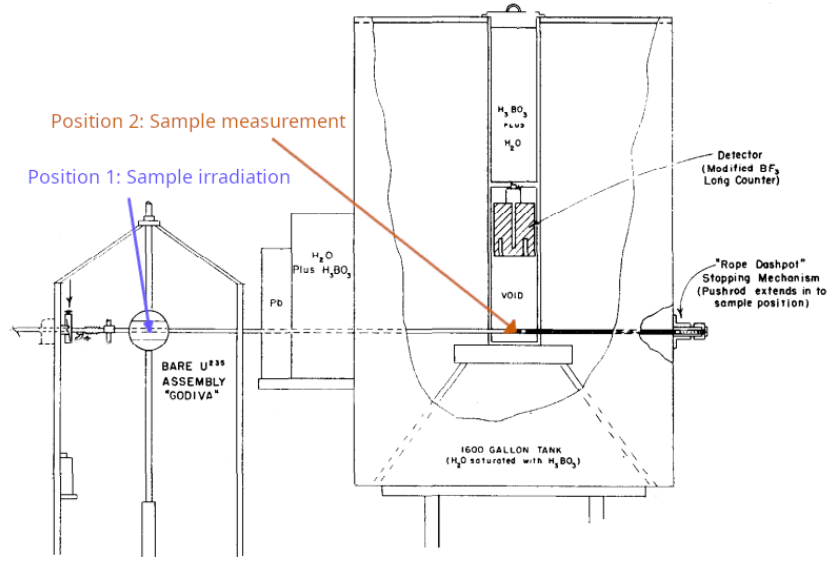
Figure 2.1: Simplified experimental setup for measuring delayed neutron emission from irradiation of a 3 gram sample in Godiva referenced from [94].
